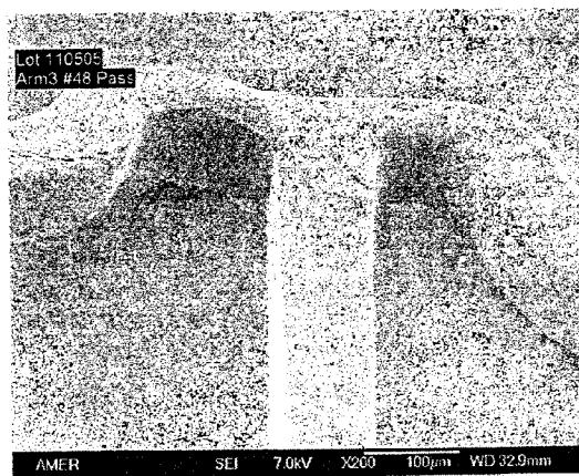
Figure 4. ID view of PEA-TEMPO - LeMans 100 ug system post-simulated use and ETO sterilization.
