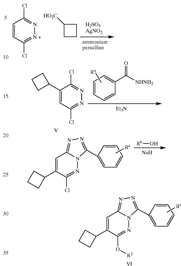
Reaction Scheme 2
