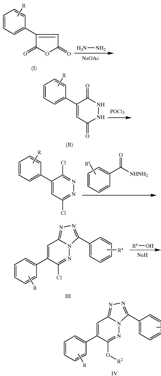
Reaction Scheme 1
