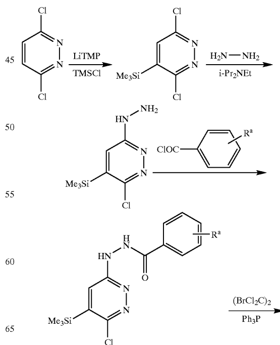
Reaction Scheme 3
