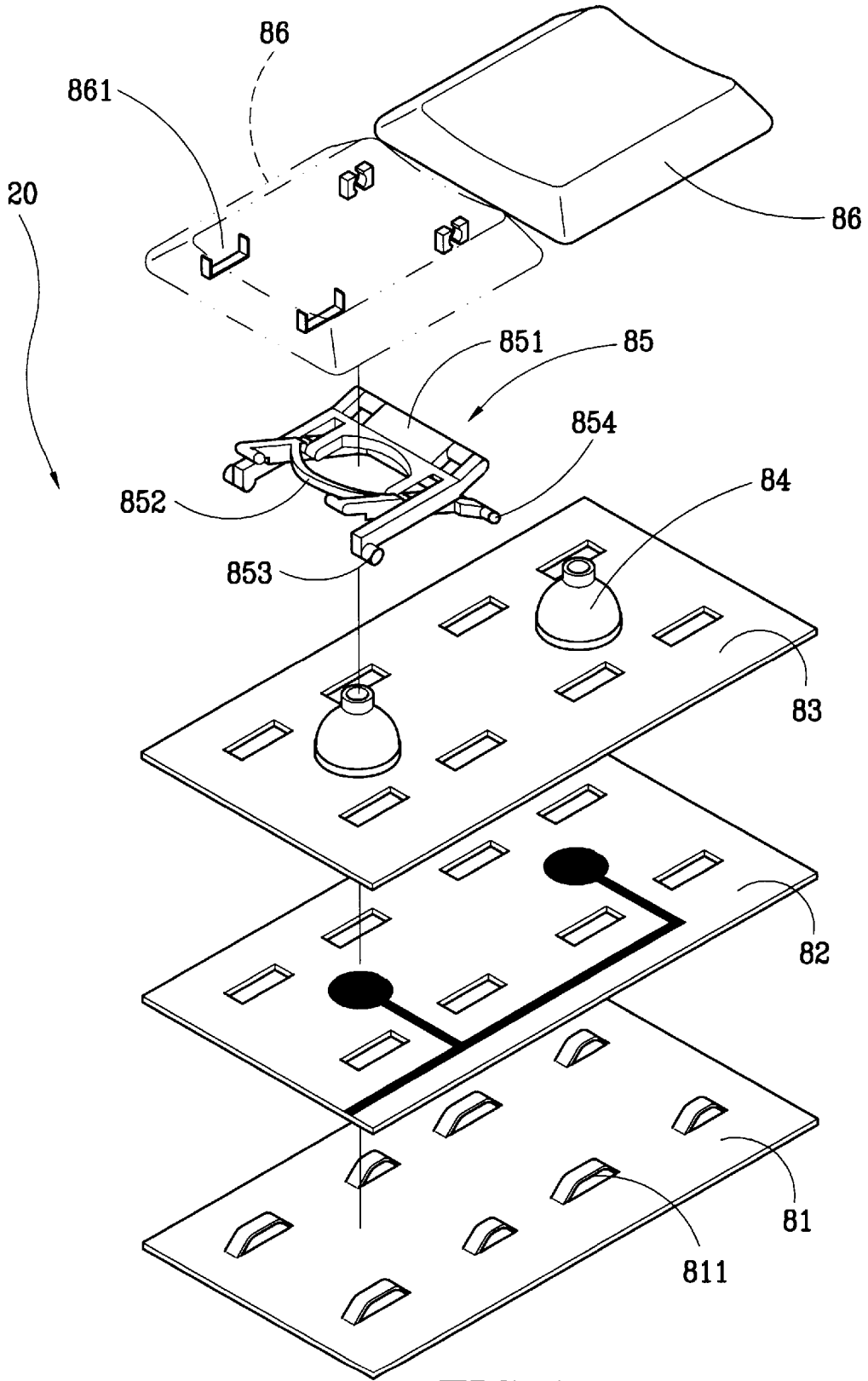
FIG.4 PRIOR ART
