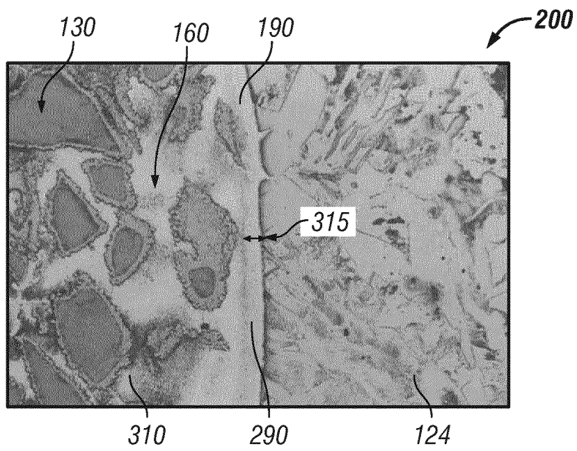
FIG. 3 (Prior Art)
