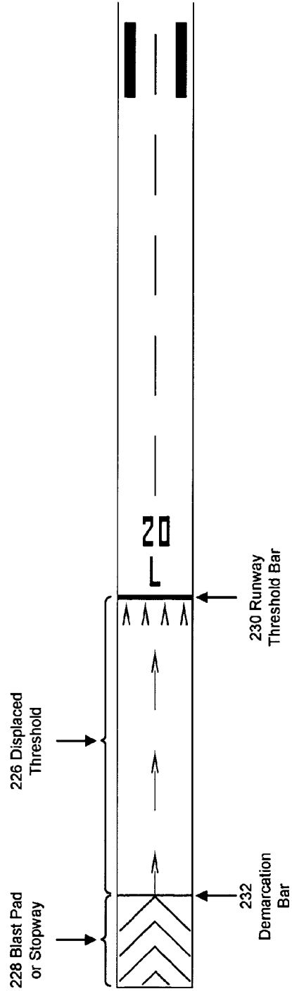
Non-Runway Markings FIG. 4D
