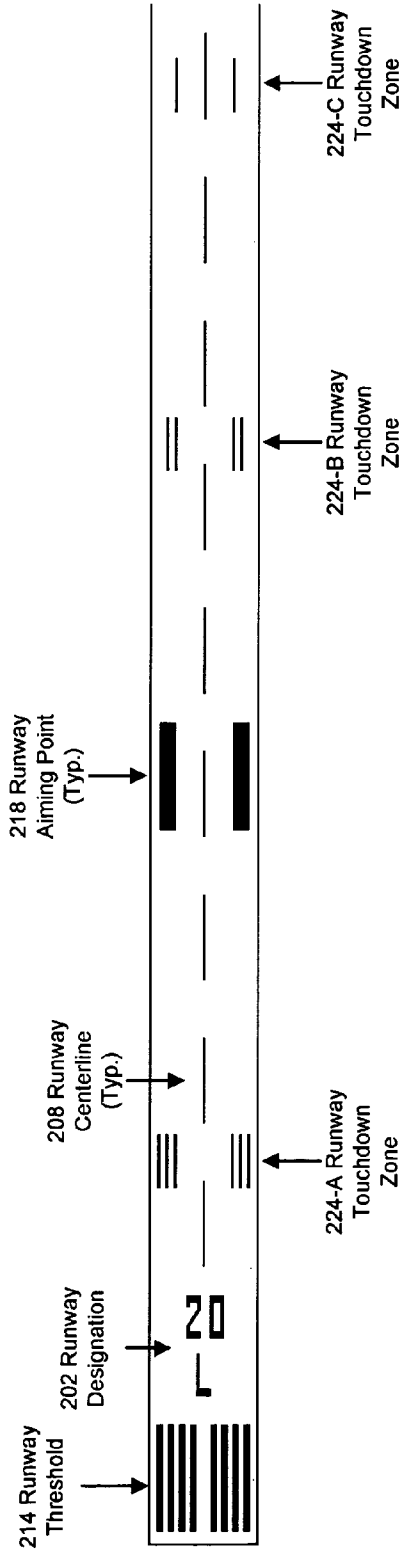
Precision Runway Markings FIG. 4A
