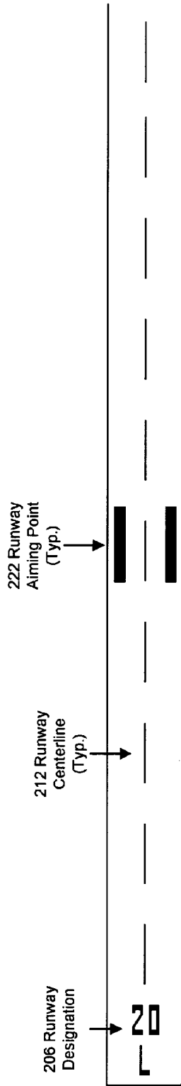
Visual Runway Markings FIG. 4C
