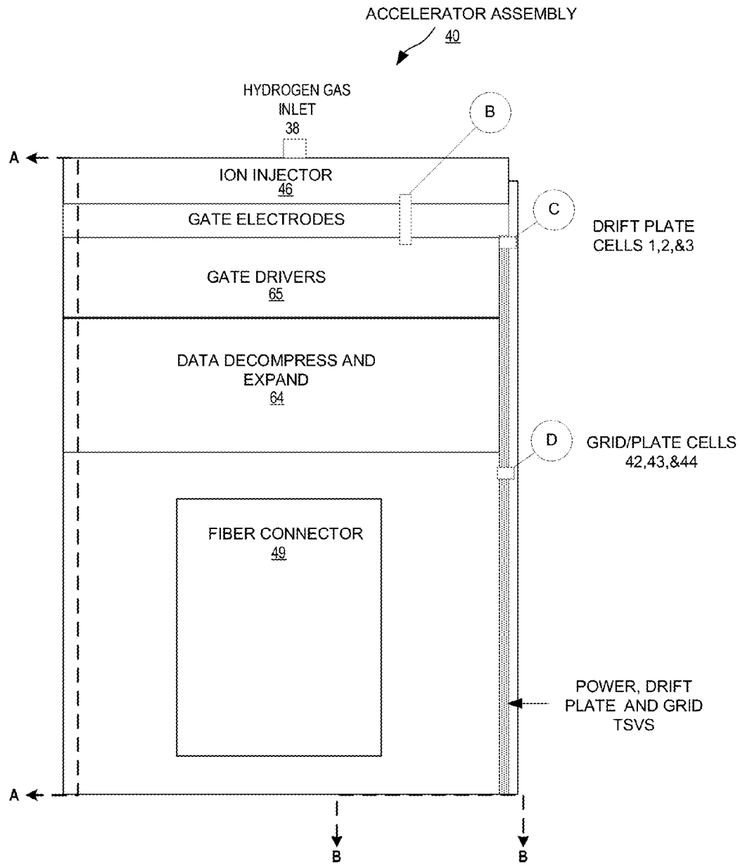
ACCELERATOR ASSEMBLY FIG. 16
