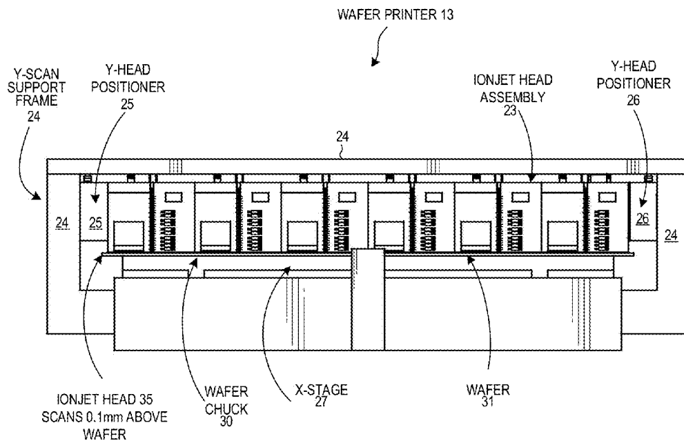
WAFER PRINTER (SIDE VIEW)
