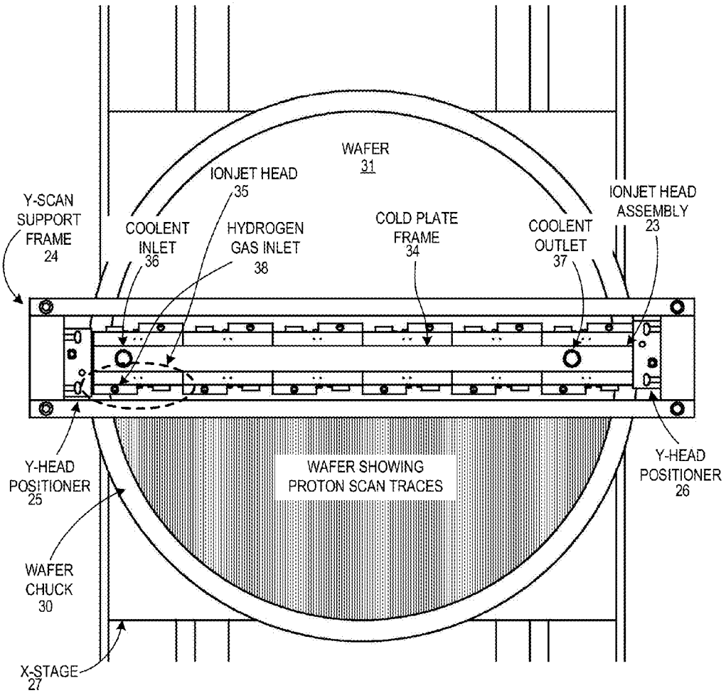
WAFER PRINTER (TOP-DOWN VIEW) FIG. 7
