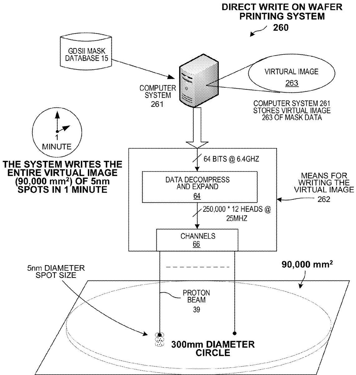
DIRECT WRITE ON WAFER PRINTING SYSTEM
