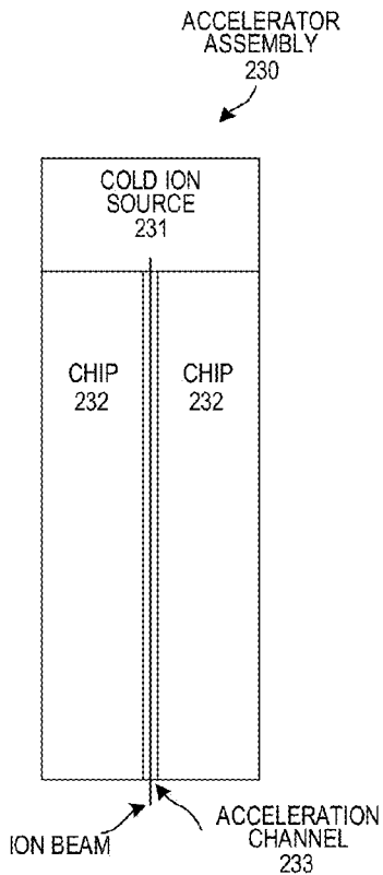
ACCELERATOR ON A CHIP HAVING A COLD ION SOURCE (TOP-DOWN VIEW)
