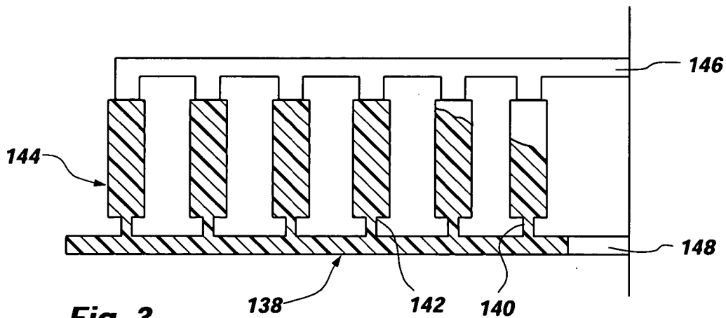
Fig. 3 (PRIOR ART)
