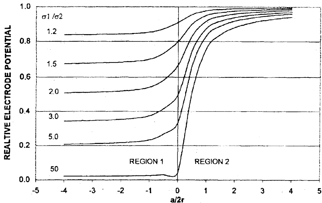
FIG.7A SPHERICAL ELECTRODE
