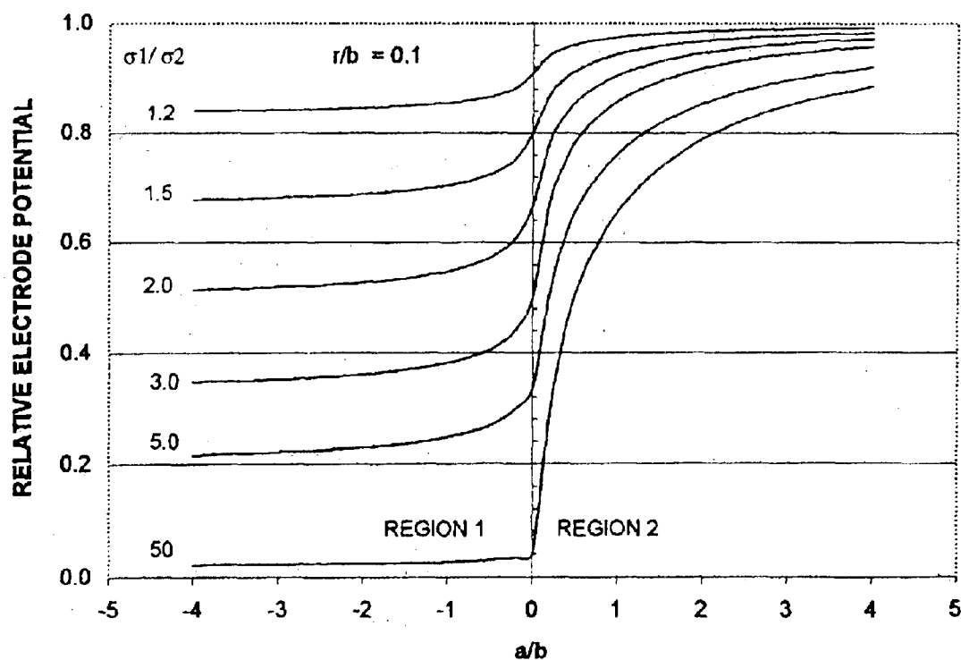
FIG.7B RING ELECTRODE
