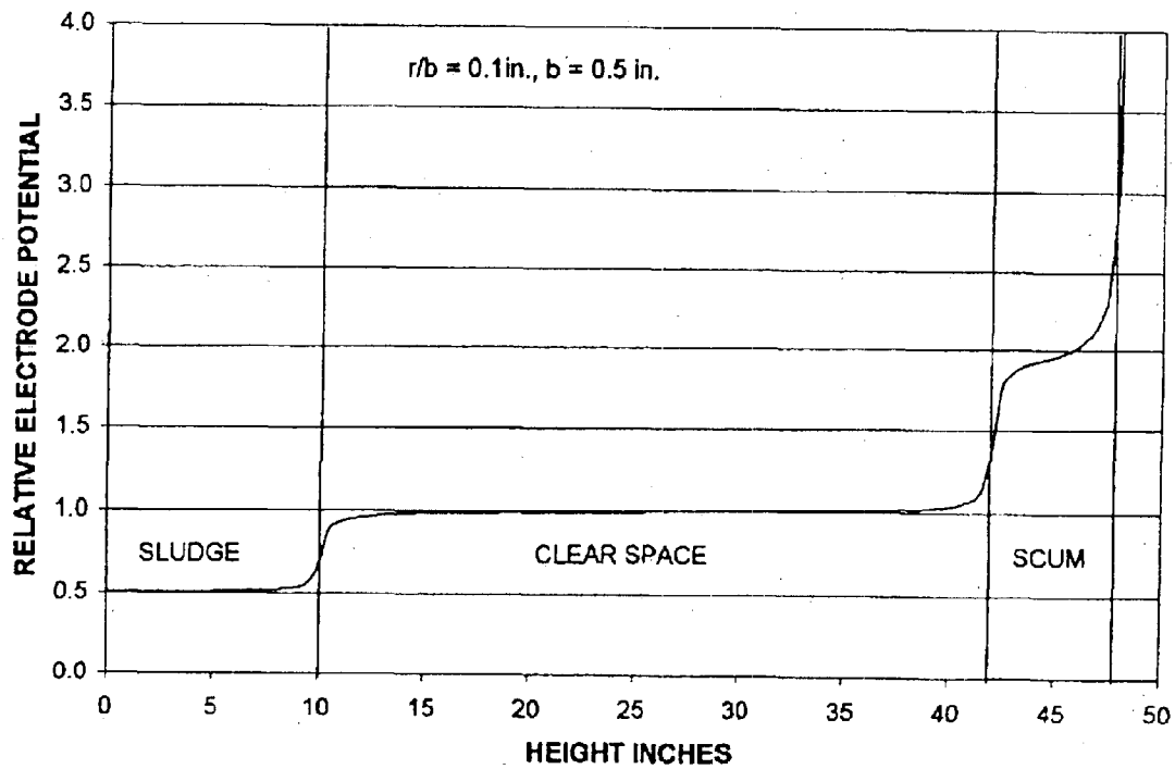
FIG. 8B RING ELECTRODE
