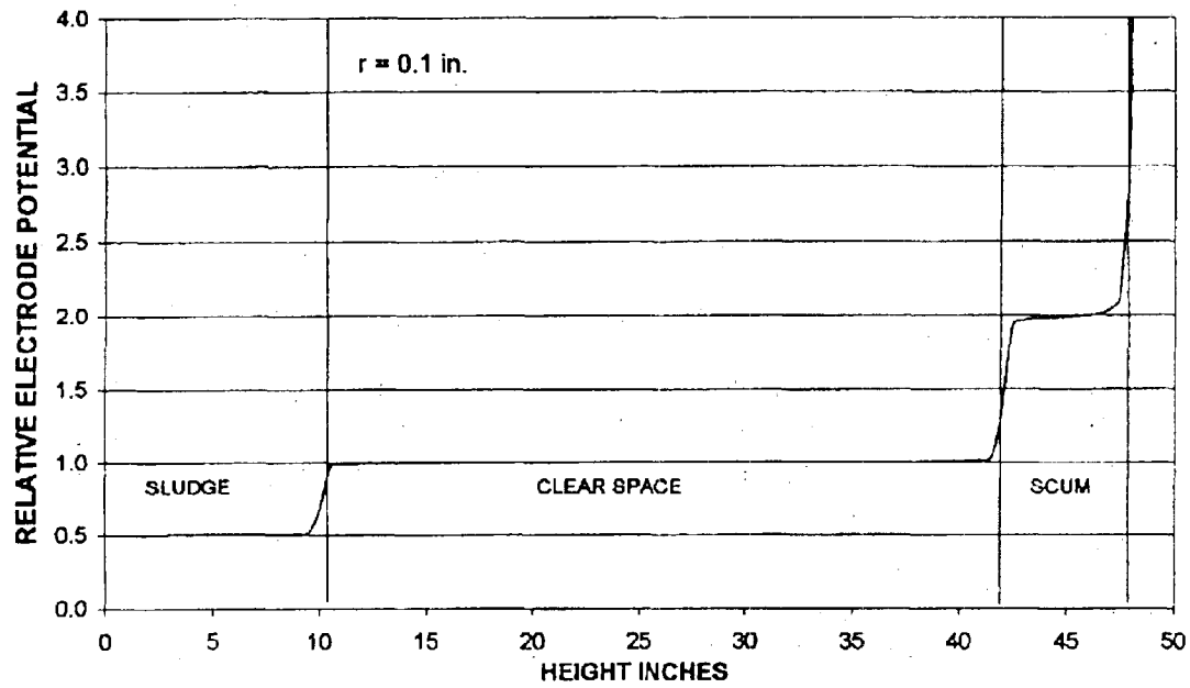
FIG. 8A SPHERICAL ELECTRODE
