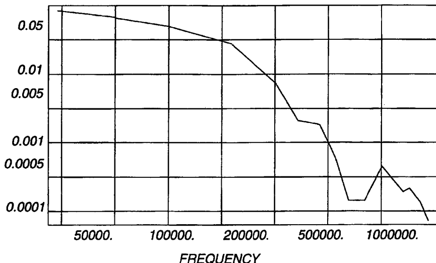
AMPLITUDE VERSUS FREQUENCY OF INTER-BUILDING UTP LOOP
