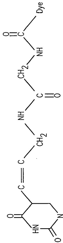
Diglycinylnyl linker
