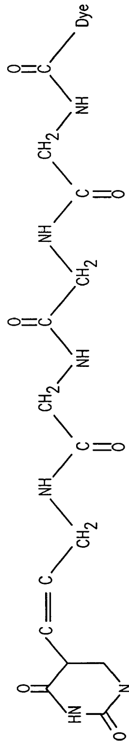
Tetraglycinylnyl linker
