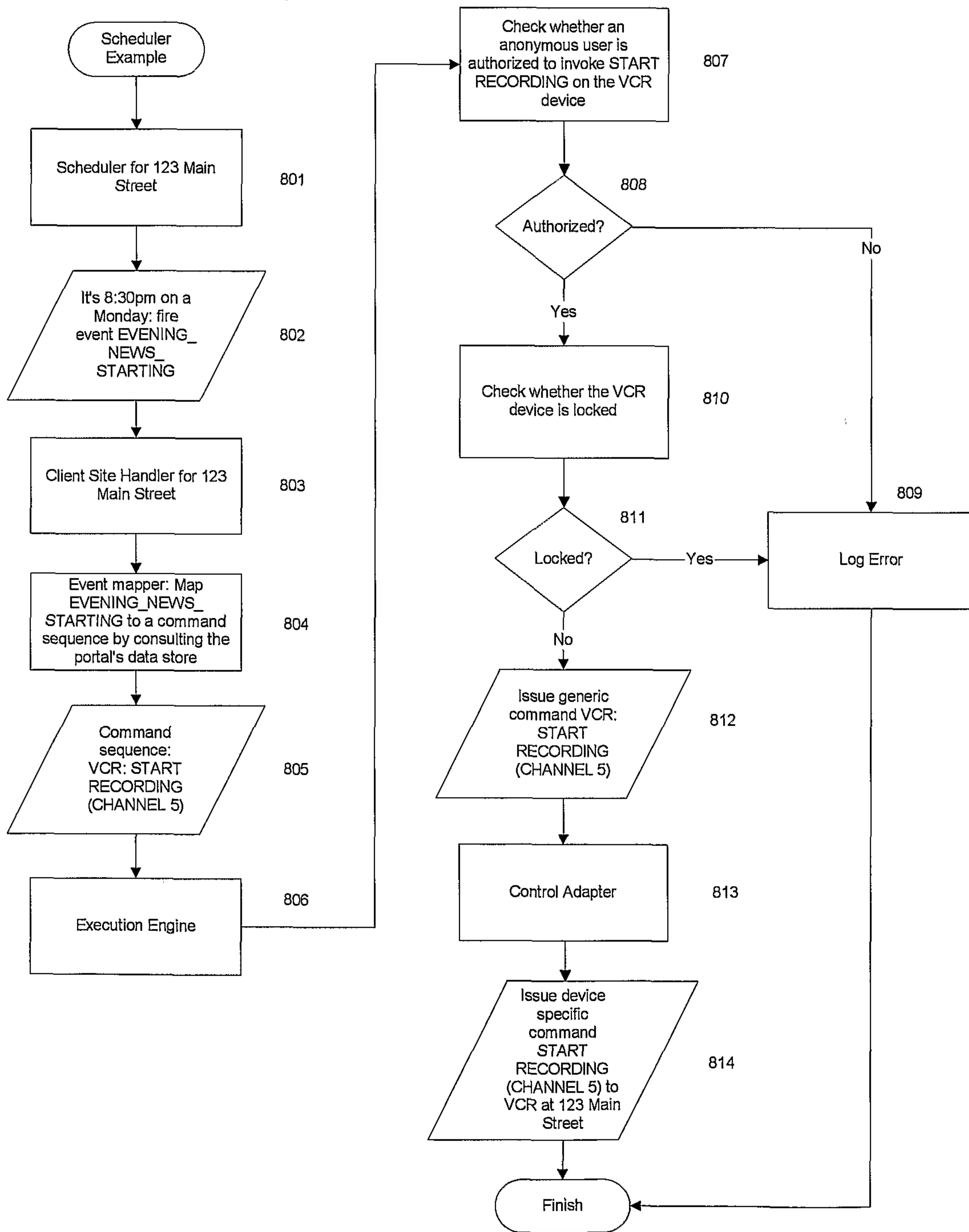
Figure 8: An example of how the central portal handles a scheduled event.
