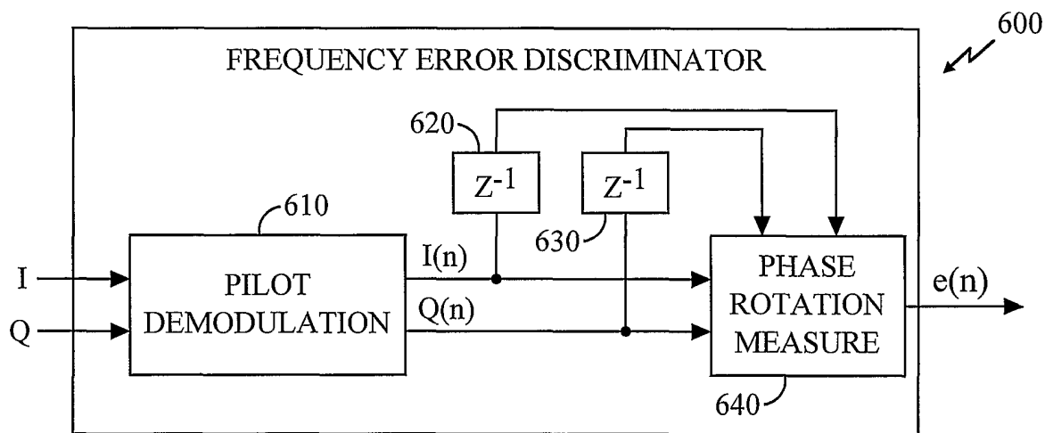
PRIOR ART FIG. 6A
