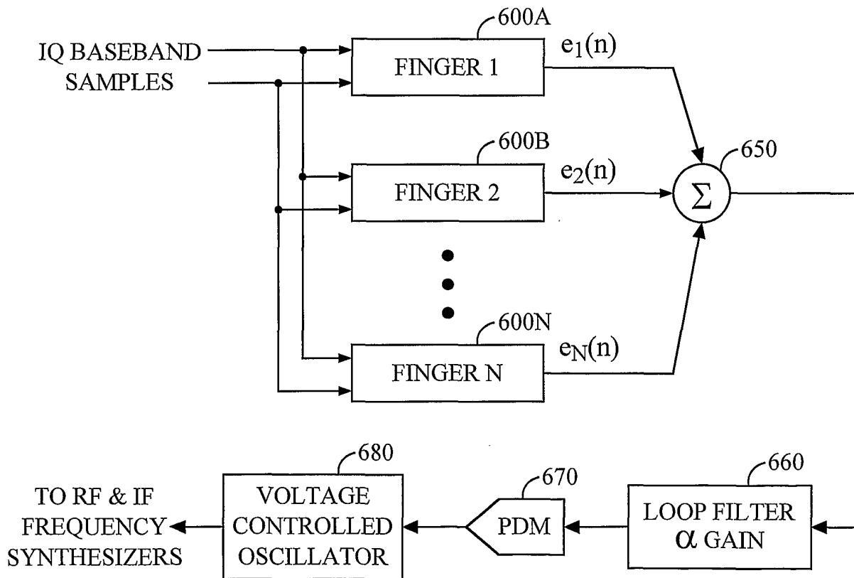
PRIOR ART FIG. 6B
