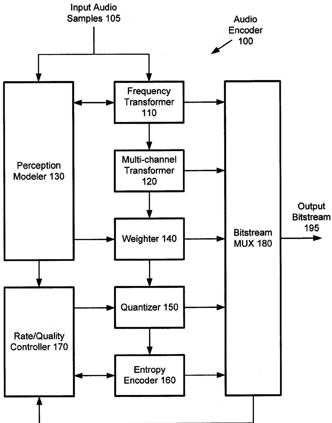
Figure 1, Prior Art
