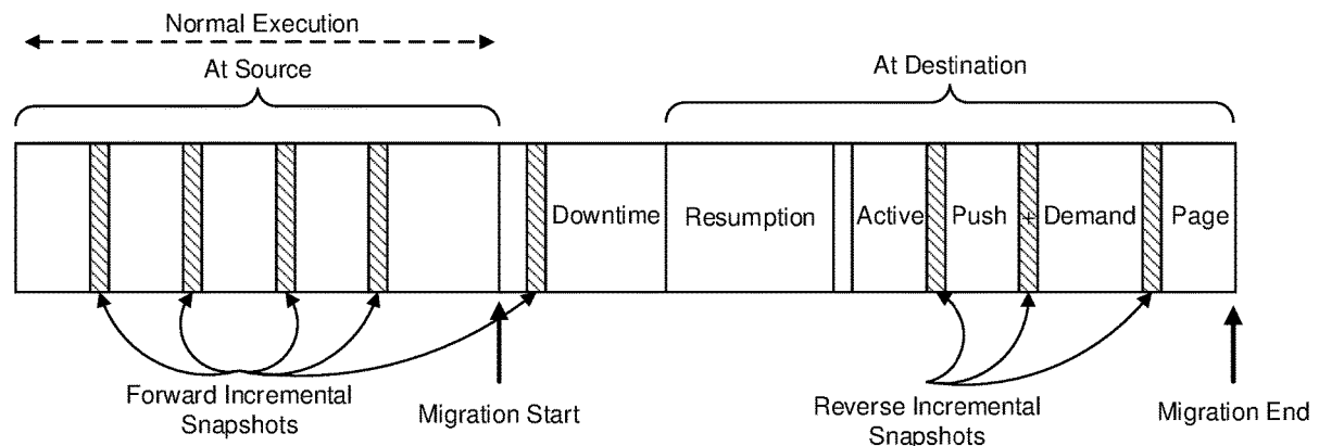
Timeline of PostCopyFT Migrations.
