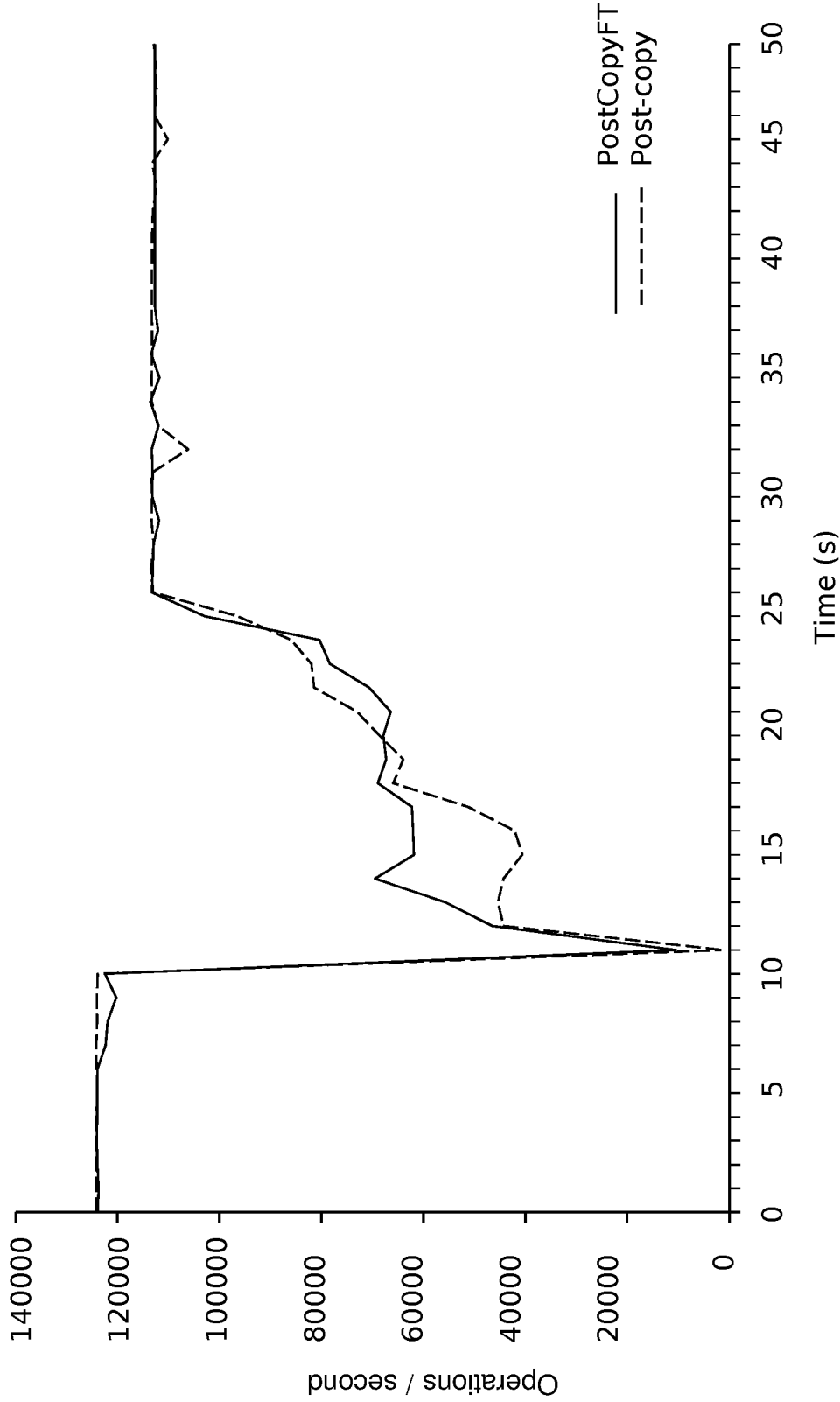
Fig. 10. The performance impact of post-copy and PostCopyFT on a CPU-intensive QuickSort benchmark.
