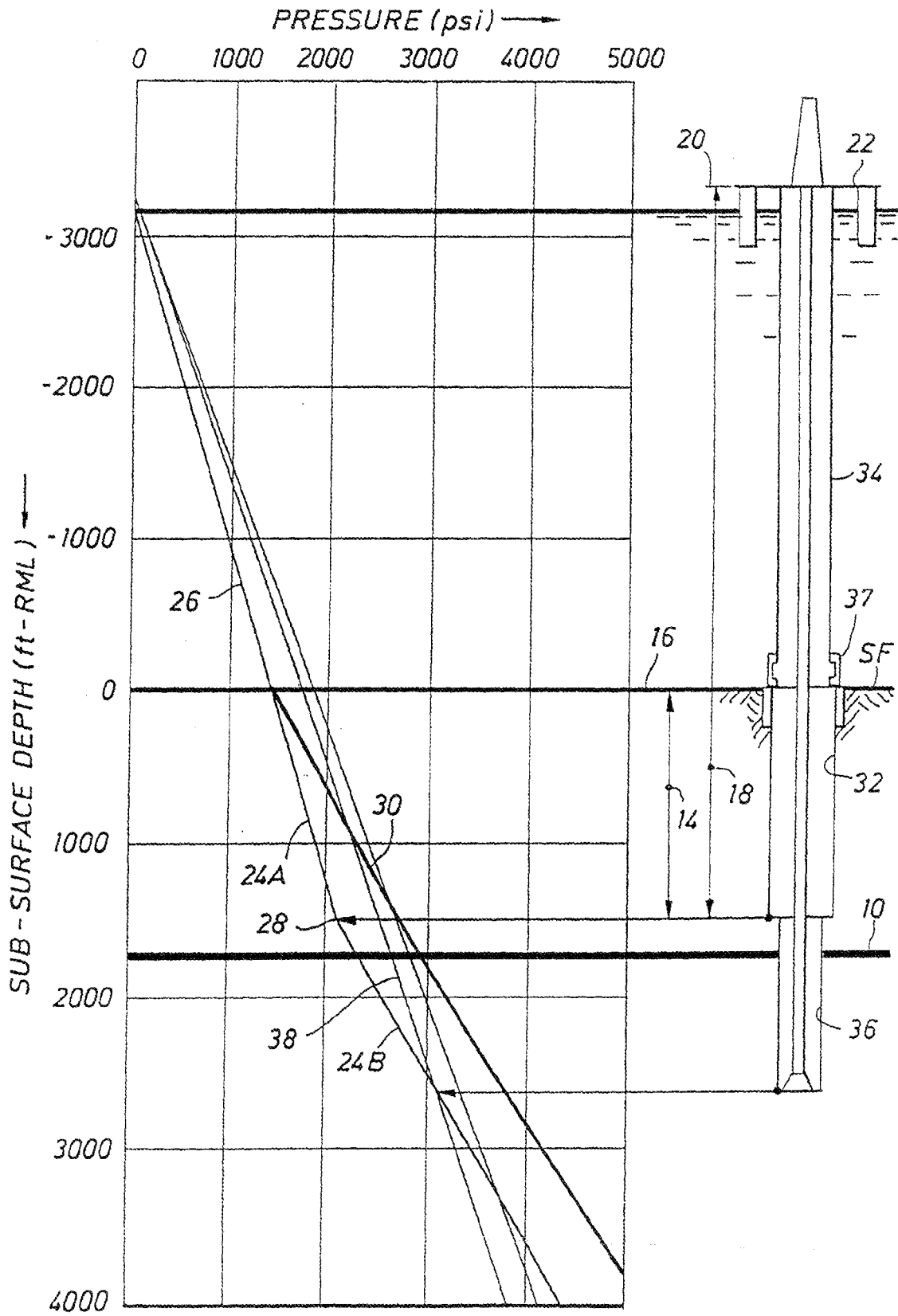
FIG.2 (PRIOR ART)
