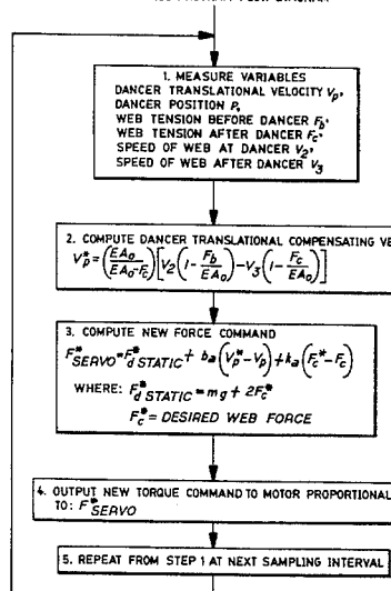
CONTROL PROGRAM FLOW DIAGRAM
