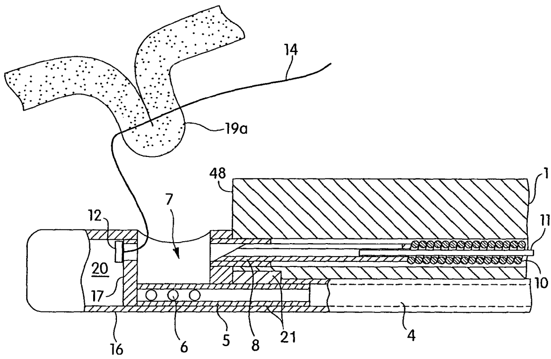
Fig. 3 (PRIOR ART)
