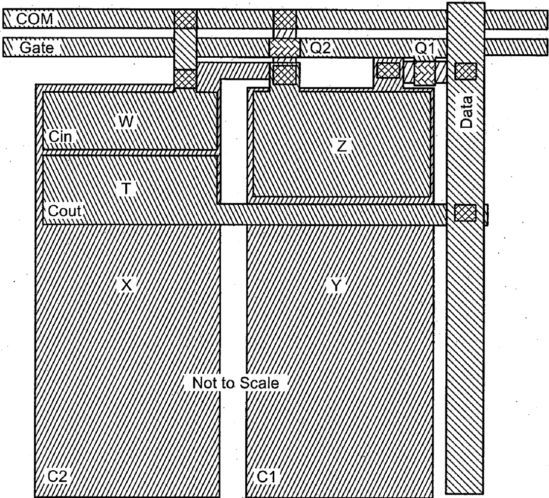
Subpixel Layout
