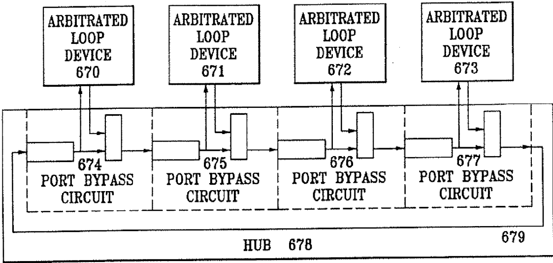
FIG. 22 (PRIOR ART)
