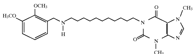
6513 1-[11-(2,3-Dimethoxybenzylamino)undecyl]-3,7-dimethylxanthine
