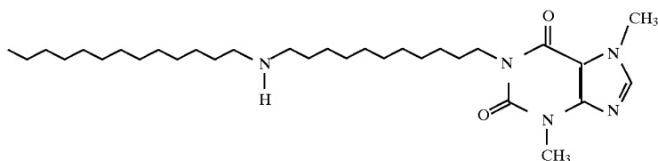
4507 1-(11-Tridecylaminoundecyl)-3,7-dimethylxanthine
