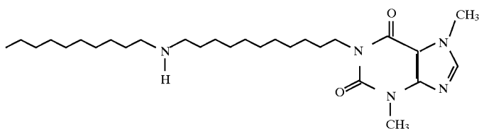
3581 1-(11-Decylaminoundecyl)-3,7-dimethylxanthine
