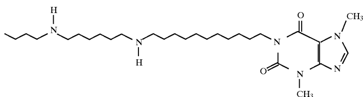
6557 1-(11-[6-(3-Butylaminohexylamino)undecyl]-3,7-dimethylxanthine
