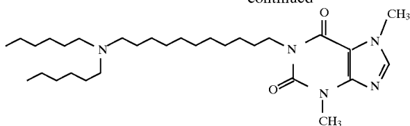
3590 1-[11-(N,N-Dihexylamino)undecyl]-3,6-dimethylxanthine
