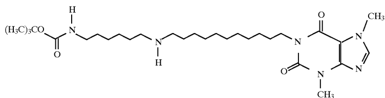
6555 1-(11-[6-(3-Tert-butoxyaminohexylamino)undecyl]-3,7-dimethylxanthine
