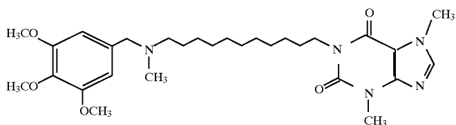
6576 1-(11-Dodecylethylaminoundecyl)-3,7-dimethylxanthine
