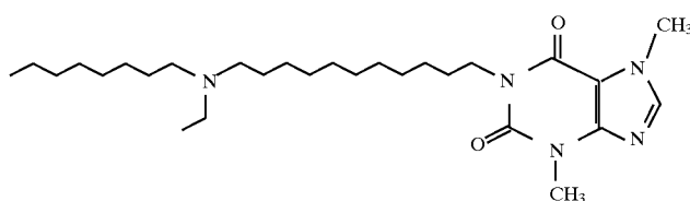
6534 1-(11-Ethyl-octylaminoundecyl)-3,7-dimethylxanthine
