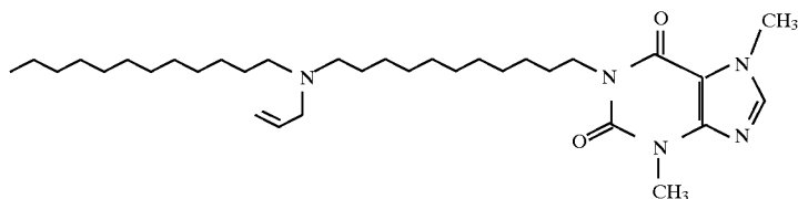
6563 1-(11-Allyldodecylaminoundecyl)-3,7-dimethylxanthine
