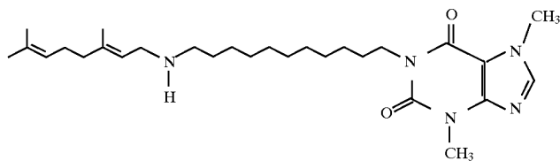
6579 1-[11-(trans-3,7-Dimethyl-2,6-octadienylamino)undecyl]-3,7-dimethylxanthine
