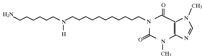
6556 1-(11-[6-(3-Aminohexylamino)undecyl]-3,7-dimethylxanthine
