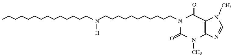
3582 1-(11-Tetradecylaminoundecyl)-3,7-dimethylxanthine
