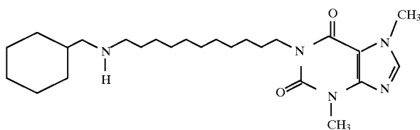
6542 1-[11-(Cyclohexylmethylamino)undecyl]-3,7-dimethylxanthine
