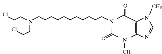
4505 1-[11-N,N-di(2-chloroethyl)aminoundecyl]-3,7-dimethylxanthine
