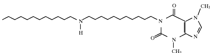
3563 1-(11-Dodecylaminoundecyl)-3,7-dimethylxanthine
