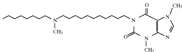
5589 1-[11-(Methyloctylamino)undecyl]-3,7-dimethylxanthine
