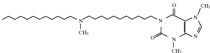
3576 1-[11-(N-Methyl-N-dodecylamino)undecyl]-3,7-dimethylxanthine
