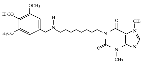
5574 1-[8-(3,4,5-Trimethoxybenzylamino)octyl]-3,7-dimethylxanthine
