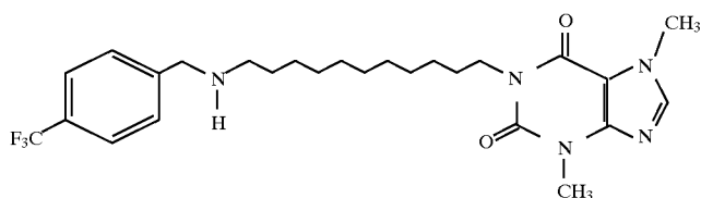
6510 1-[11-(4-Trifluoromethylbenzylamino)undecyl]-3,7-dimethylxanthine
