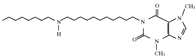
3556 1-(11-N-Octylaminoundecyl)-3,7-dimethylxanthine
