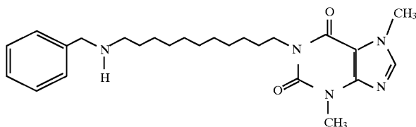
6531 1-[11-Benzylaminoundecyl]-3,7-dimethylxanthine
