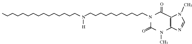
4508 1-(11-Pentadecylaminodecyl)-3,7-dimethylxanthine
