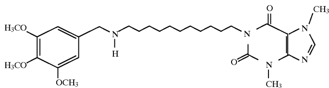
3593 1-[11-(3,4,5-Trimethoxybenzylamino)undecyl]-3,7-dimethylxanthine
