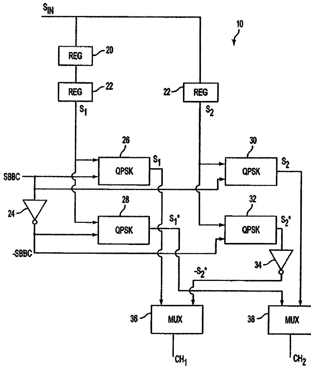
FIG. 3 (PRIOR ART)
