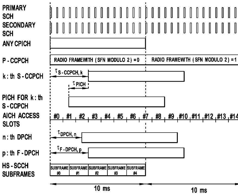
FIG. 3 (PRIOR ART)
