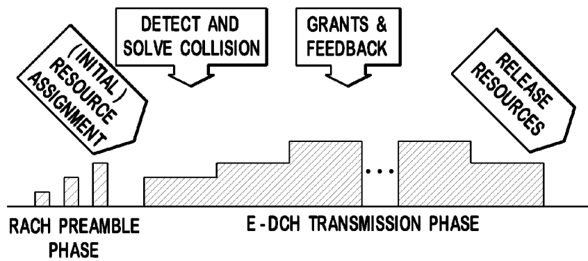
FIG. 1 (PRIOR ART)
