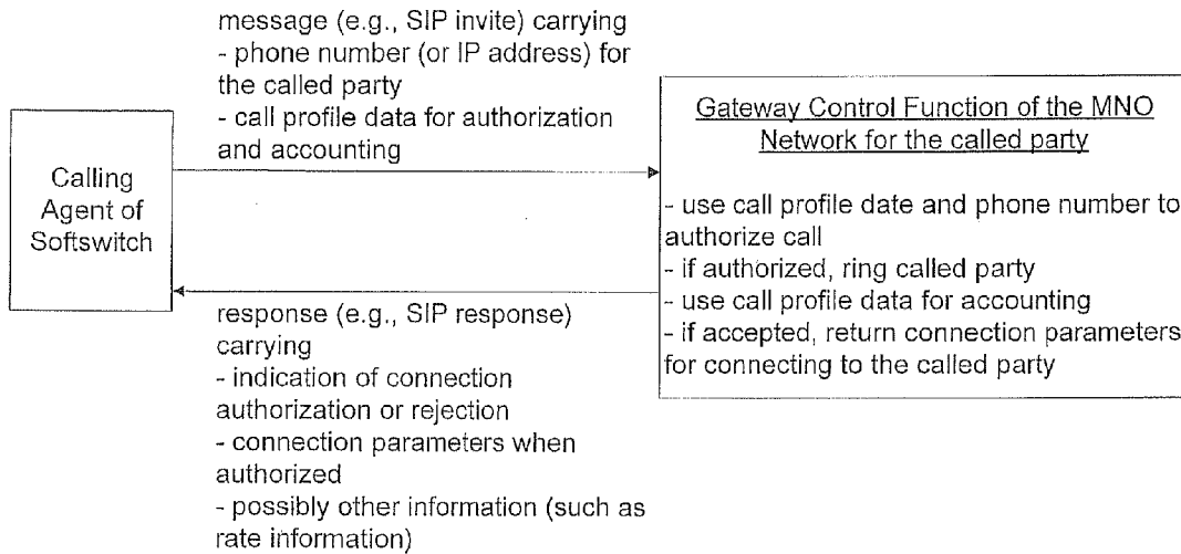
Called Party Call-Set-up Loop
