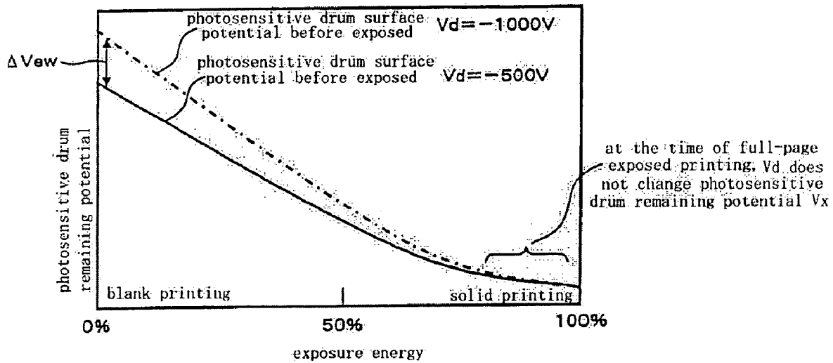
ILLUSTRATION OF RELATION BETWEEN EXPOSURE ENERGY AND PHOTOSENSITIVE DRUM REMAINING POTENTIAL
