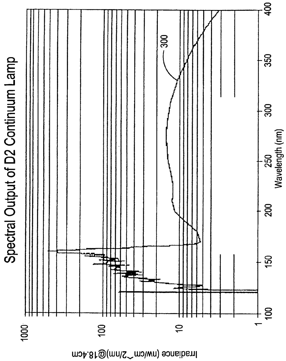
NIST Calibration (1nm Bandpass)
