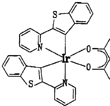
(btp) 2 Ir(acac)
