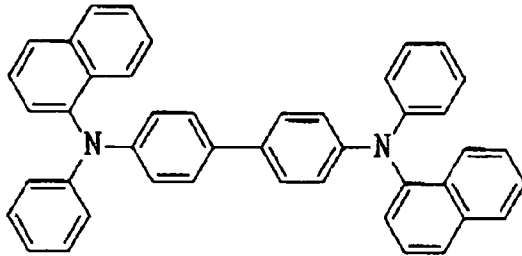
NPB
