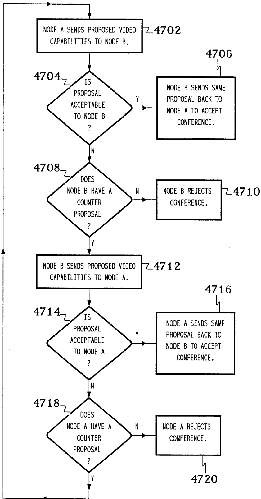
FIG. 47. VIDEO NEGOTIATION
