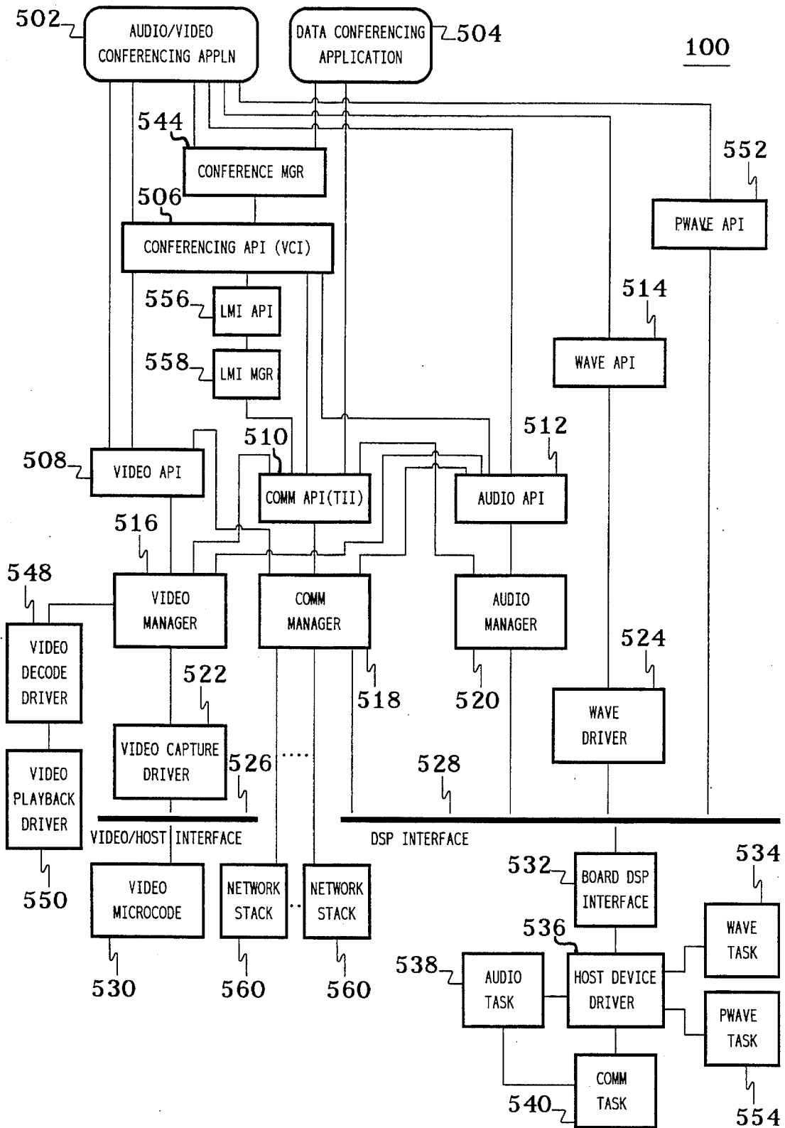
FIG. 5. CONFERENCING SYSTEM SOFTWARE ARCHITECTURE
