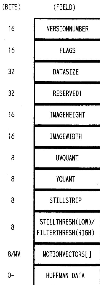
FIG. 25. COMPRESSED VIDEO DATA FIELD
