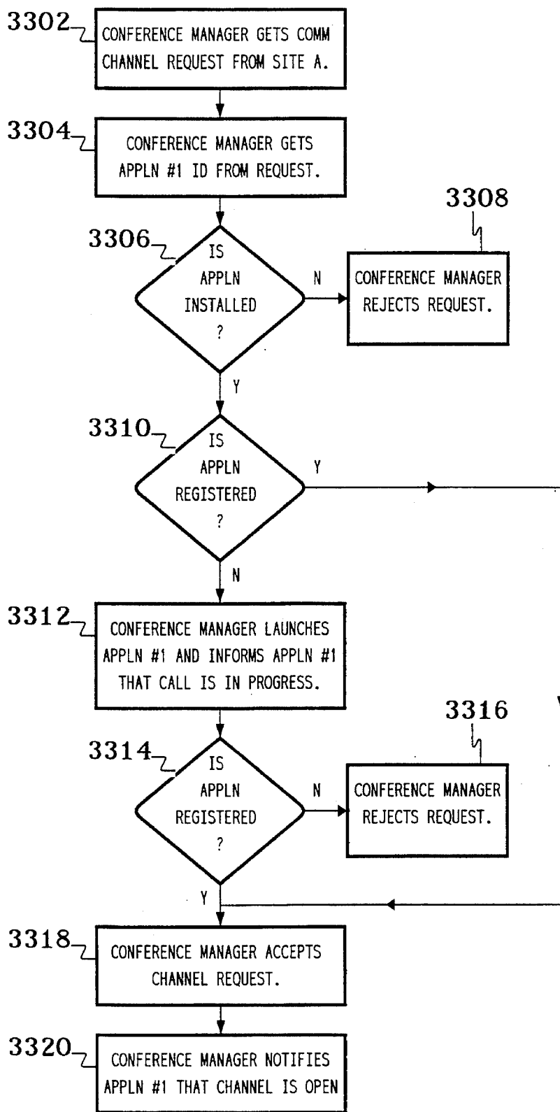
FIG. 33. ON-DEMAND INVOCATION
