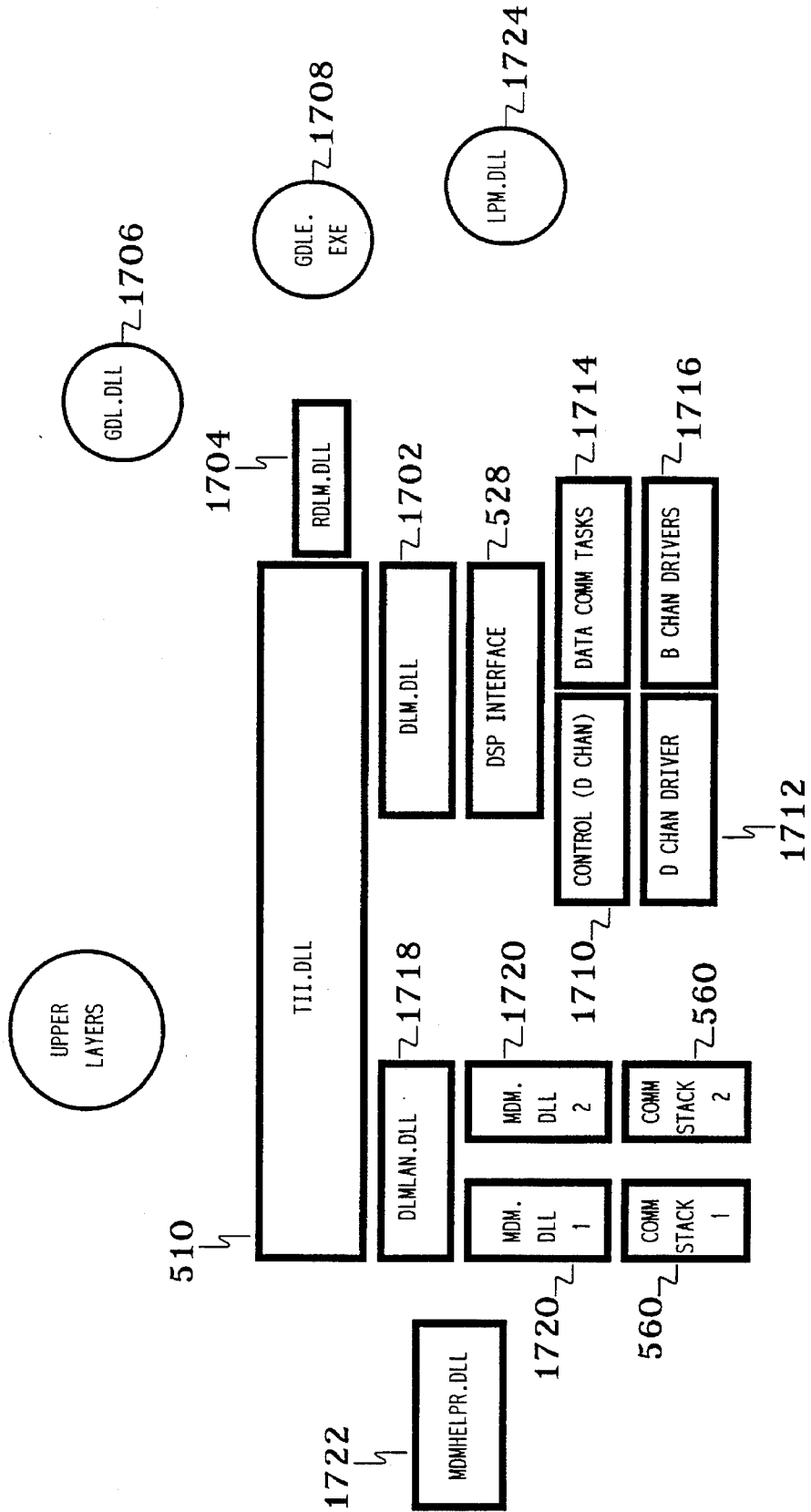
FIG. 17. COMM SUBSYSTEM LAYERS
