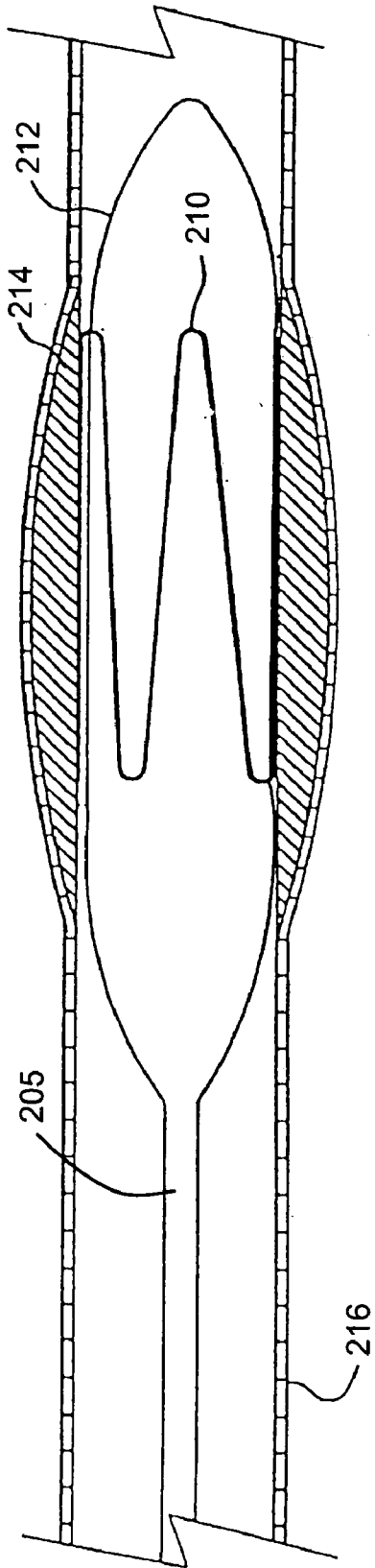
(PRIOR ART) FIG. 2A
