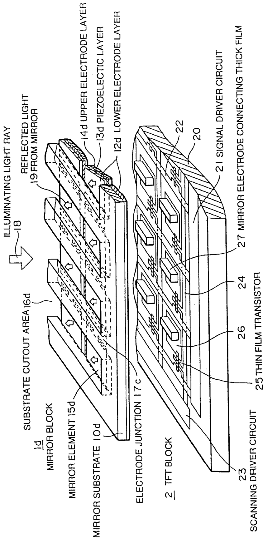
103 : OPTICAL MODULATOR DEVICE
