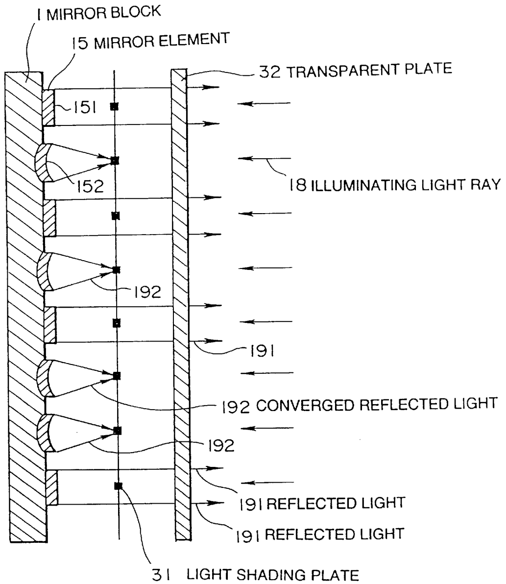
104 : OPTICAL MODULATOR DEVICE
