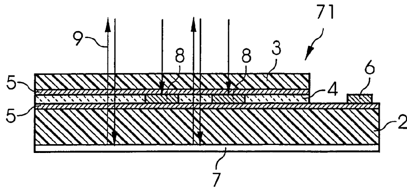
FIG 7 PRIOR ART
