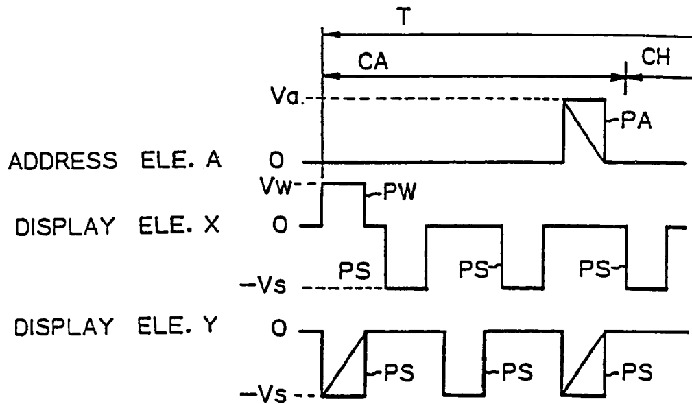
Fig. 5 PRIOR ART
