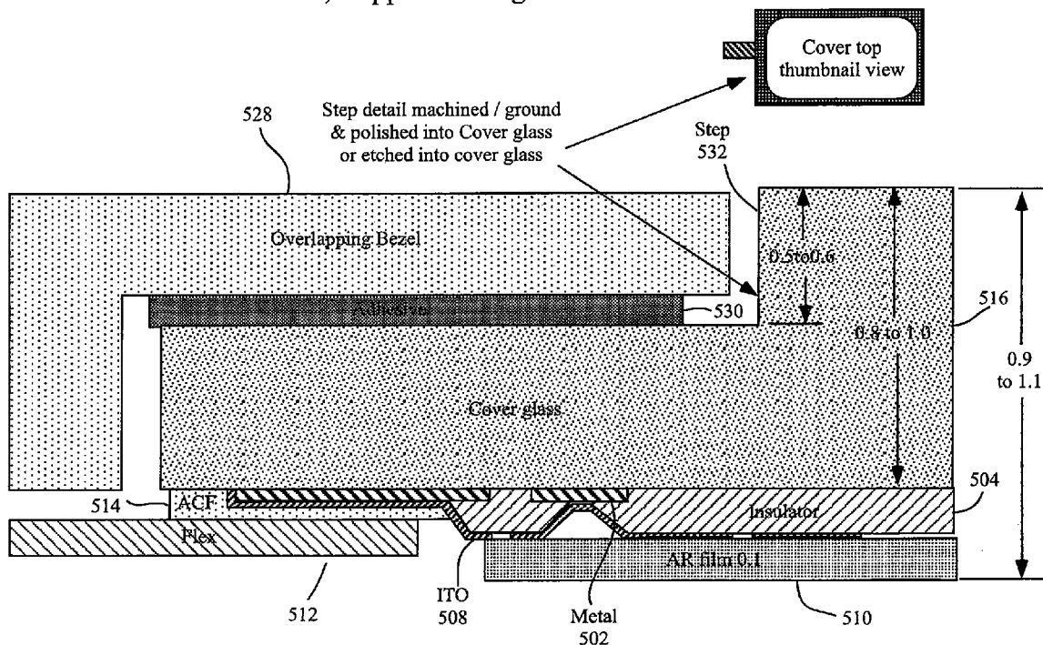
Back of cover SITO, stepped cover glass
