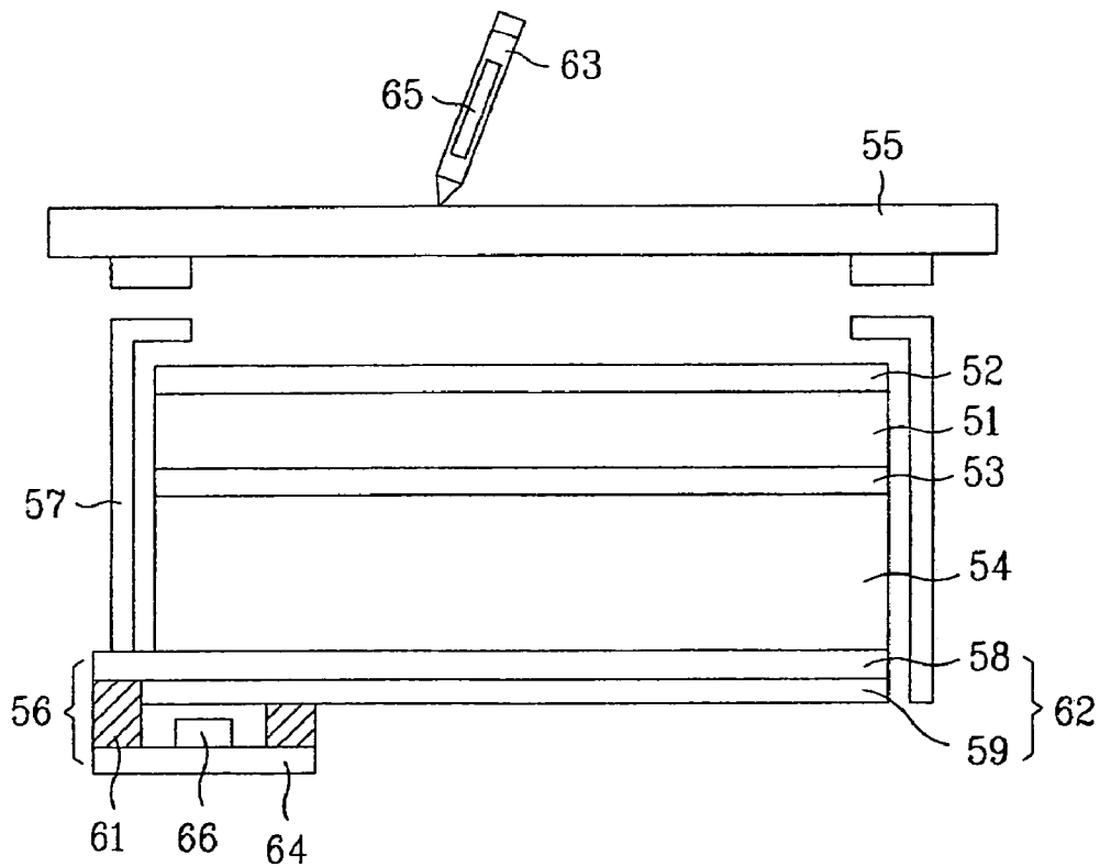
FIG. 4 Related Art
