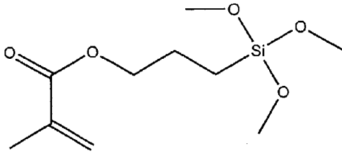
methacryloyloxypropyltrimethoxy silane
