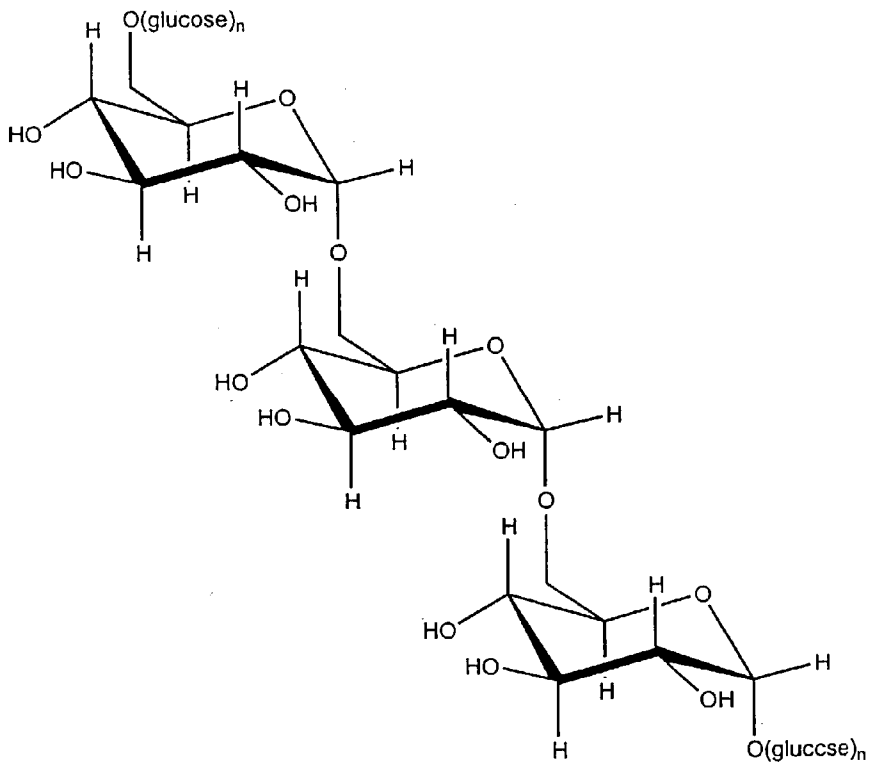
Dextran
