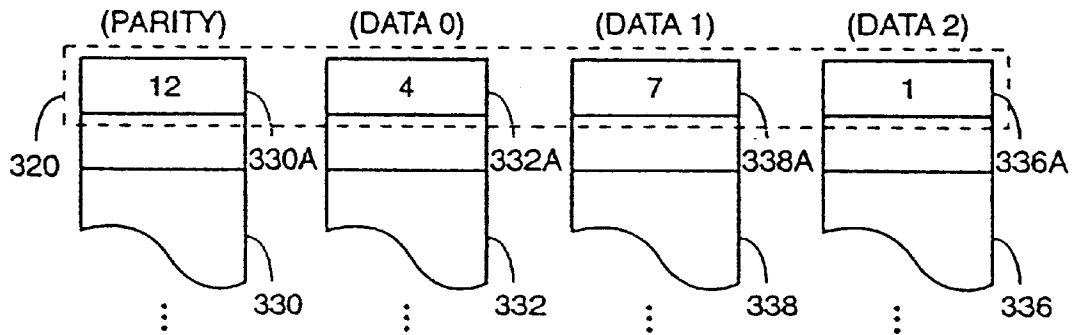
FIG. 3C (PRIOR ART)
