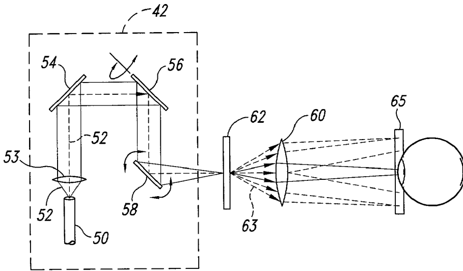
Fig. 3 (Prior Art)
