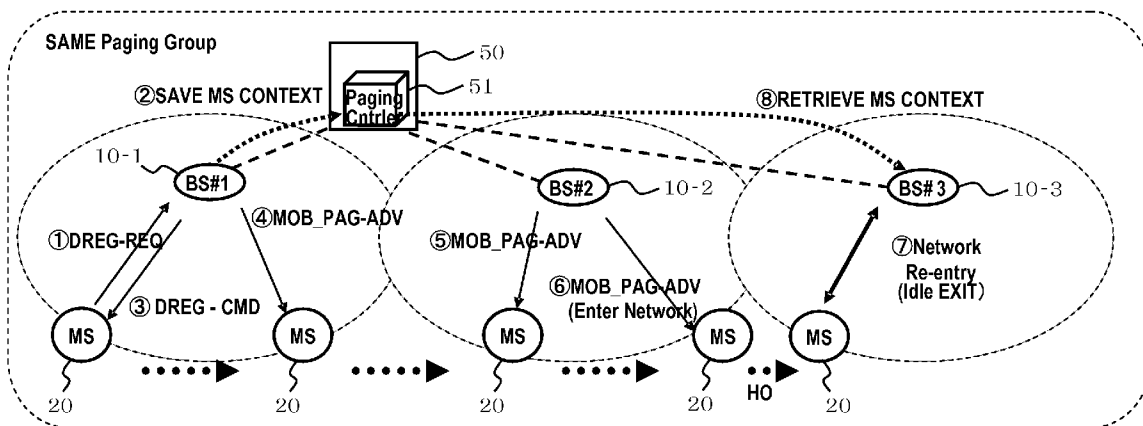
RADIO COMMUNICATION SYSTEM 1
