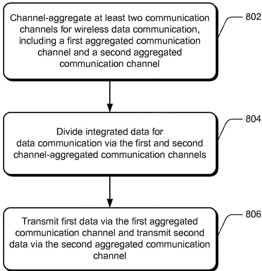
Example of Communication Transmission with Aggregated Channels
