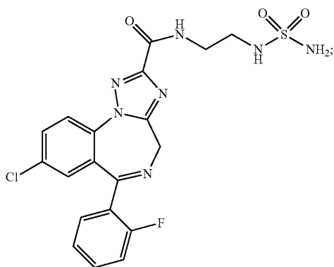
(Compound 10)
