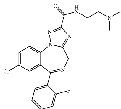
(Compound 3)
