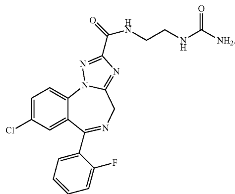
(Compound 6)
