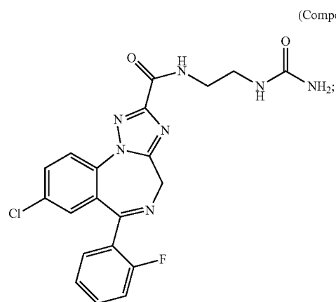
(Compound 7)
