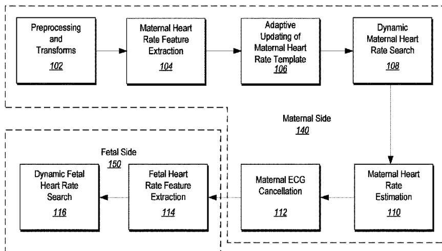
Abdominal Electrocardiogram Processing System Block Diagram Overview
