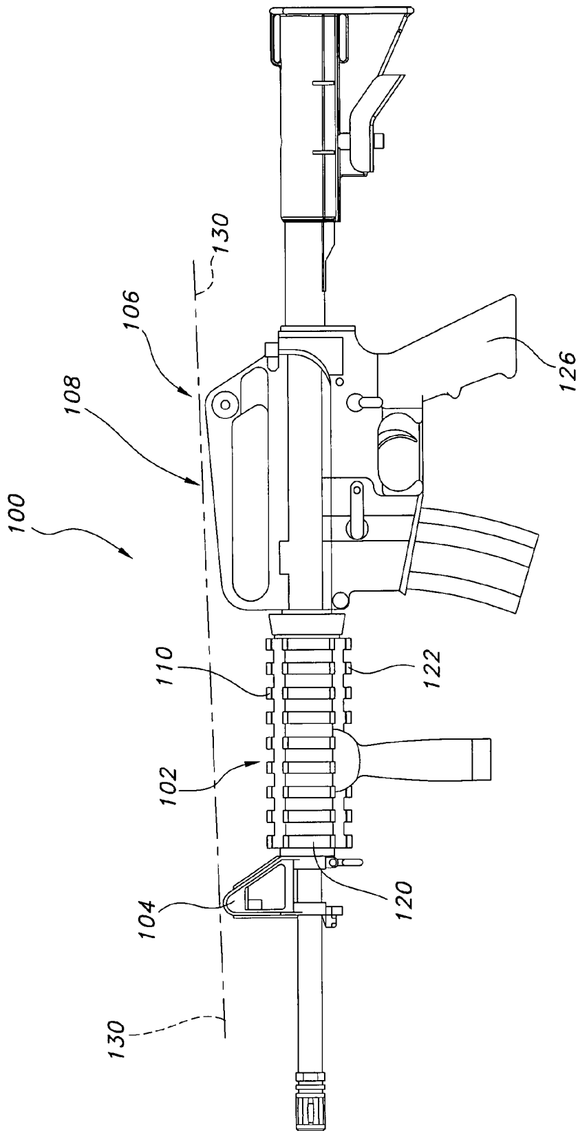
FIG. 1 (PRIOR ART)
