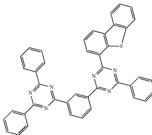
Compound 38
