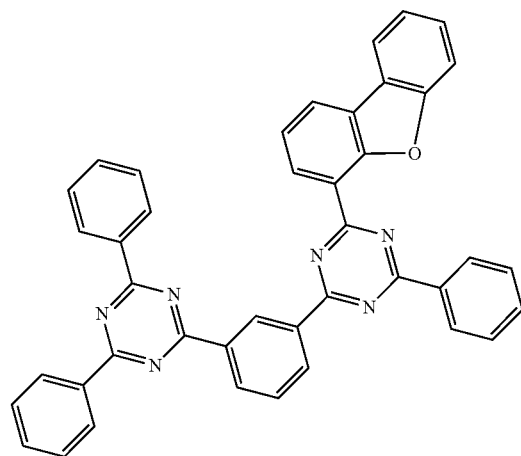
Compound 38
