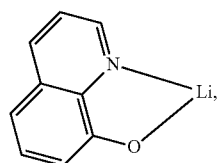
LiQ
