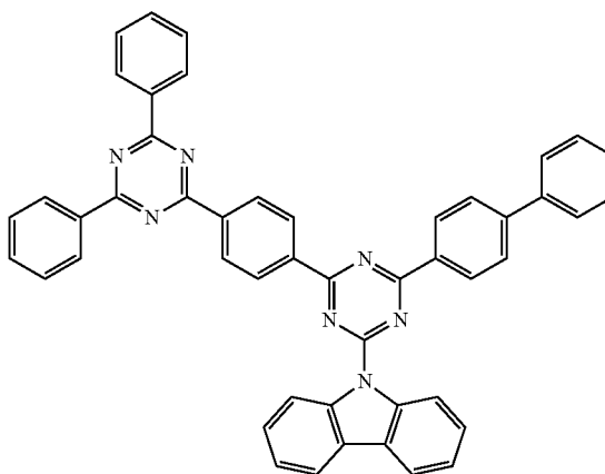
Compound 40
