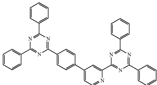
Compound 17
