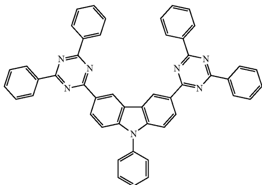
-continued Compound 3
