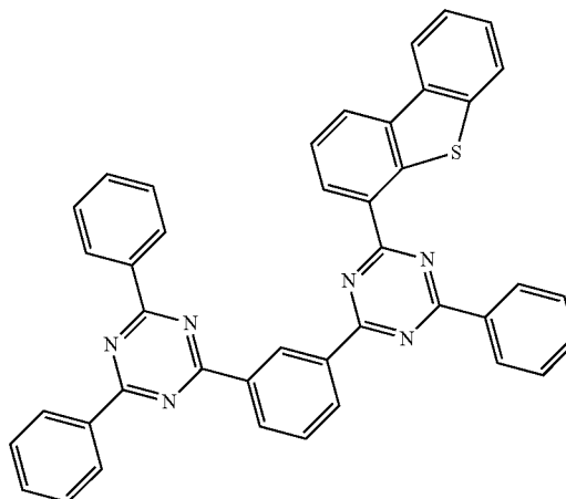
Compound 39
