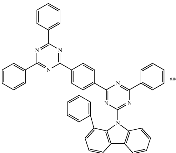
Compound 42
