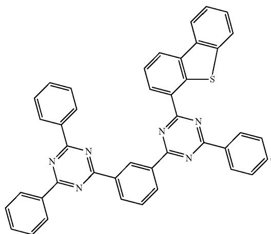
Compound 37
