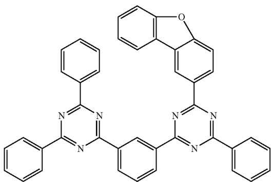
Compound 36
