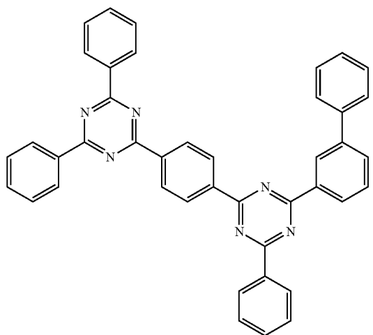
Compound 42
