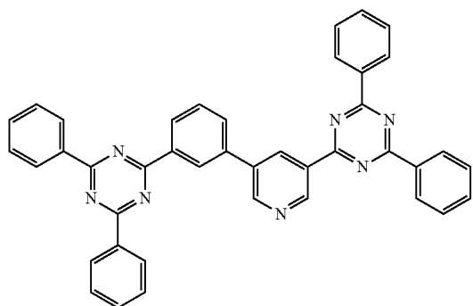
Compound 13
