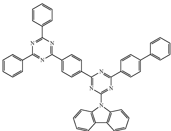
Compound 41
