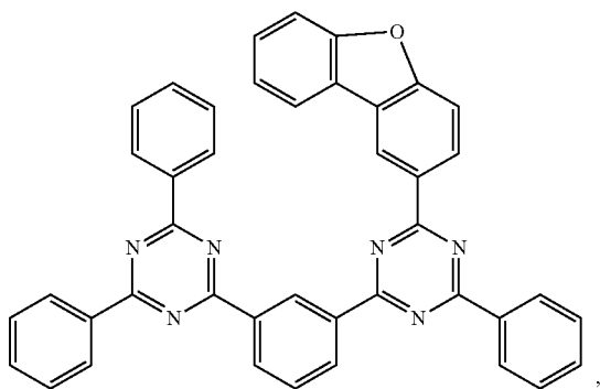
Compound 36
