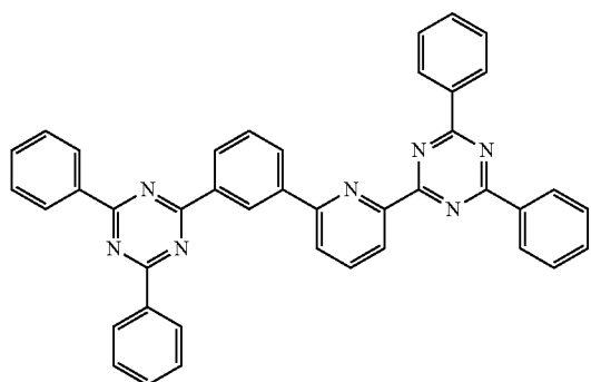
Compound 15
