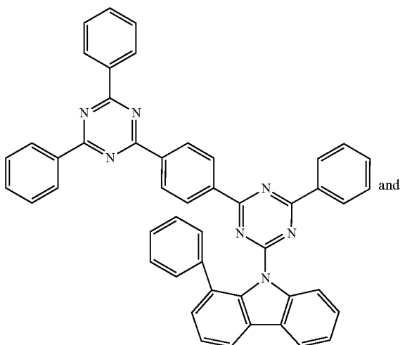
Compound 42
