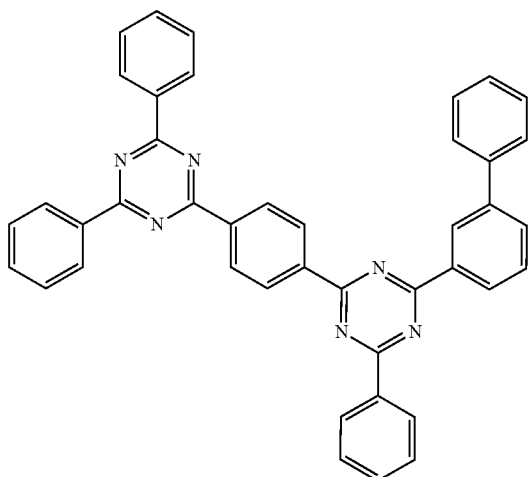
Compound 42
