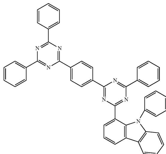
Compound 39
