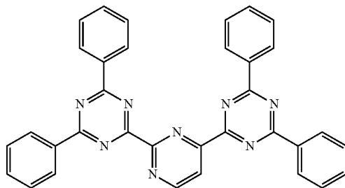
Compound 14
