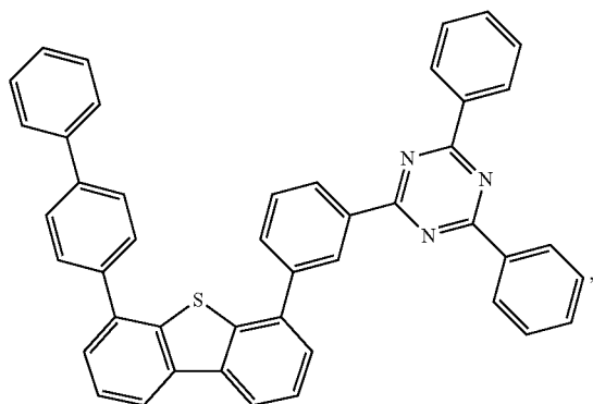
139 -continued
