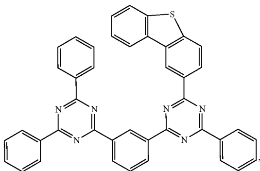
Compound 35
