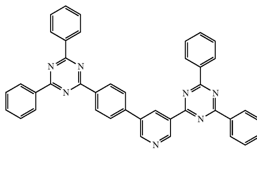
Compound 16
