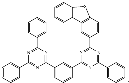
Compound 35
