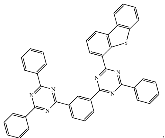
Compound 37
