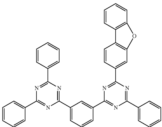
Compound 35
