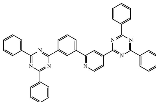
Compound 14
