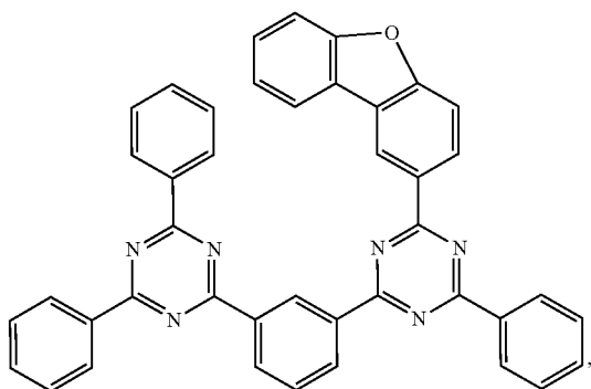
Compound 36
