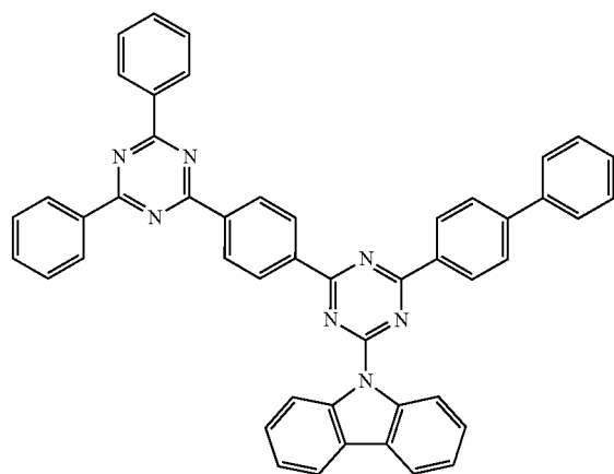
Compound 40
