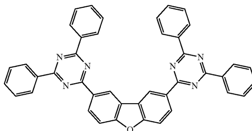
Compound 2
