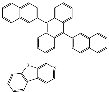
aDBT-ADN
