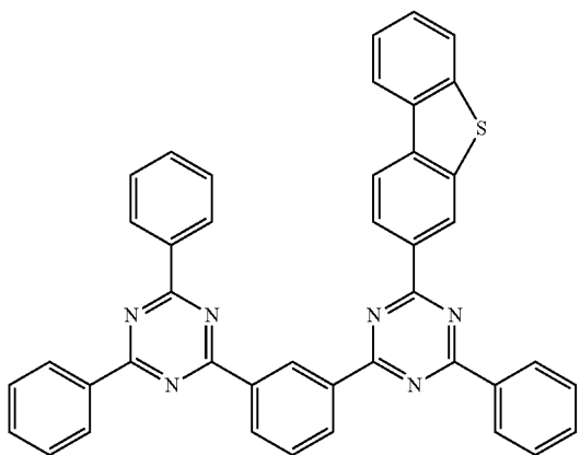
Compound 34
