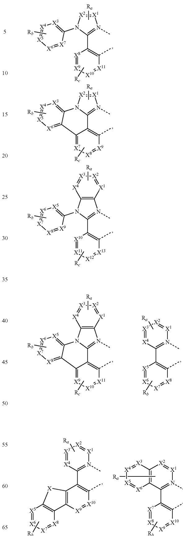
Compound 42
