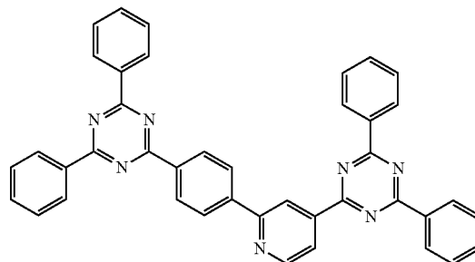
Compound 18
