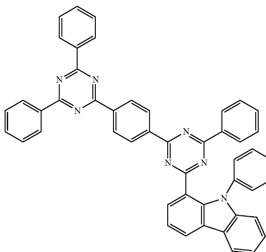
Compound 39
