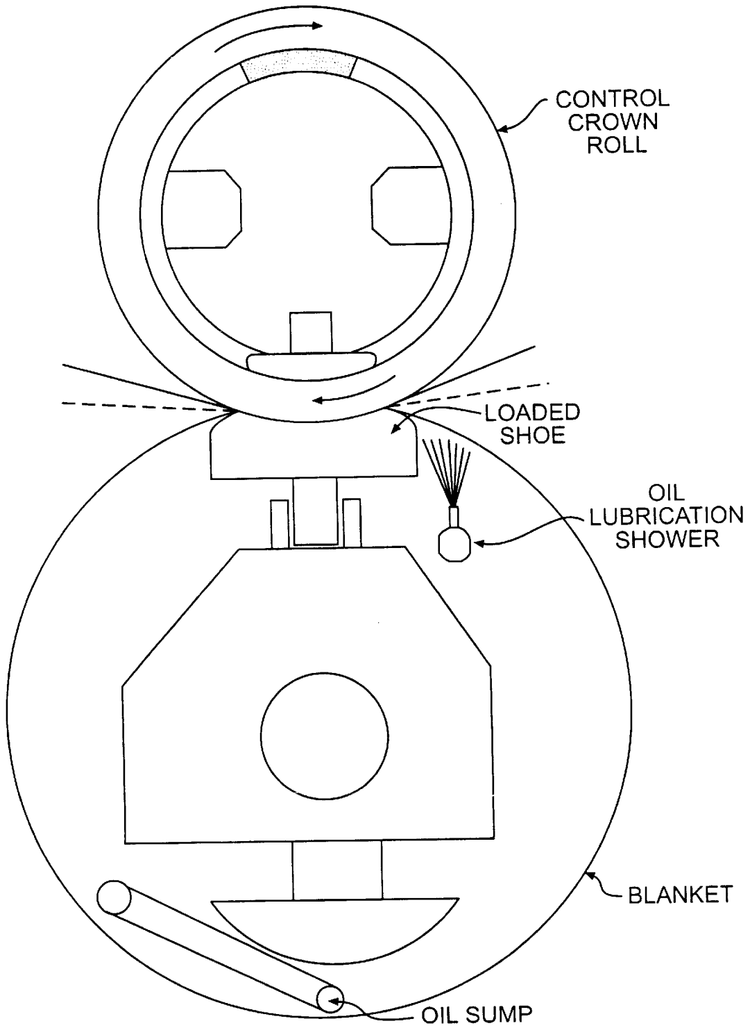
SIDE VIEW OF WIDE SHOE PRESS
