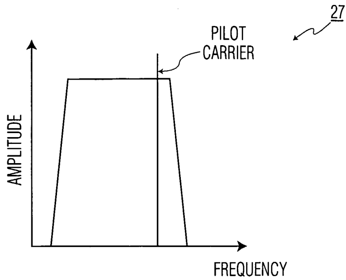
IF SIGNAL WITHOUT MULTIPATH DISTORTION
