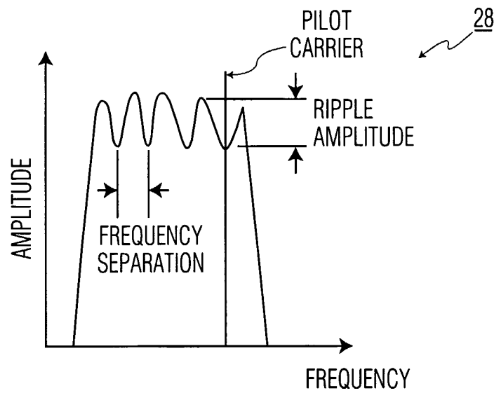
IF SIGNAL WITH MULTIPATH DISTORTION
