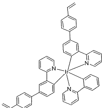
Compound 1
