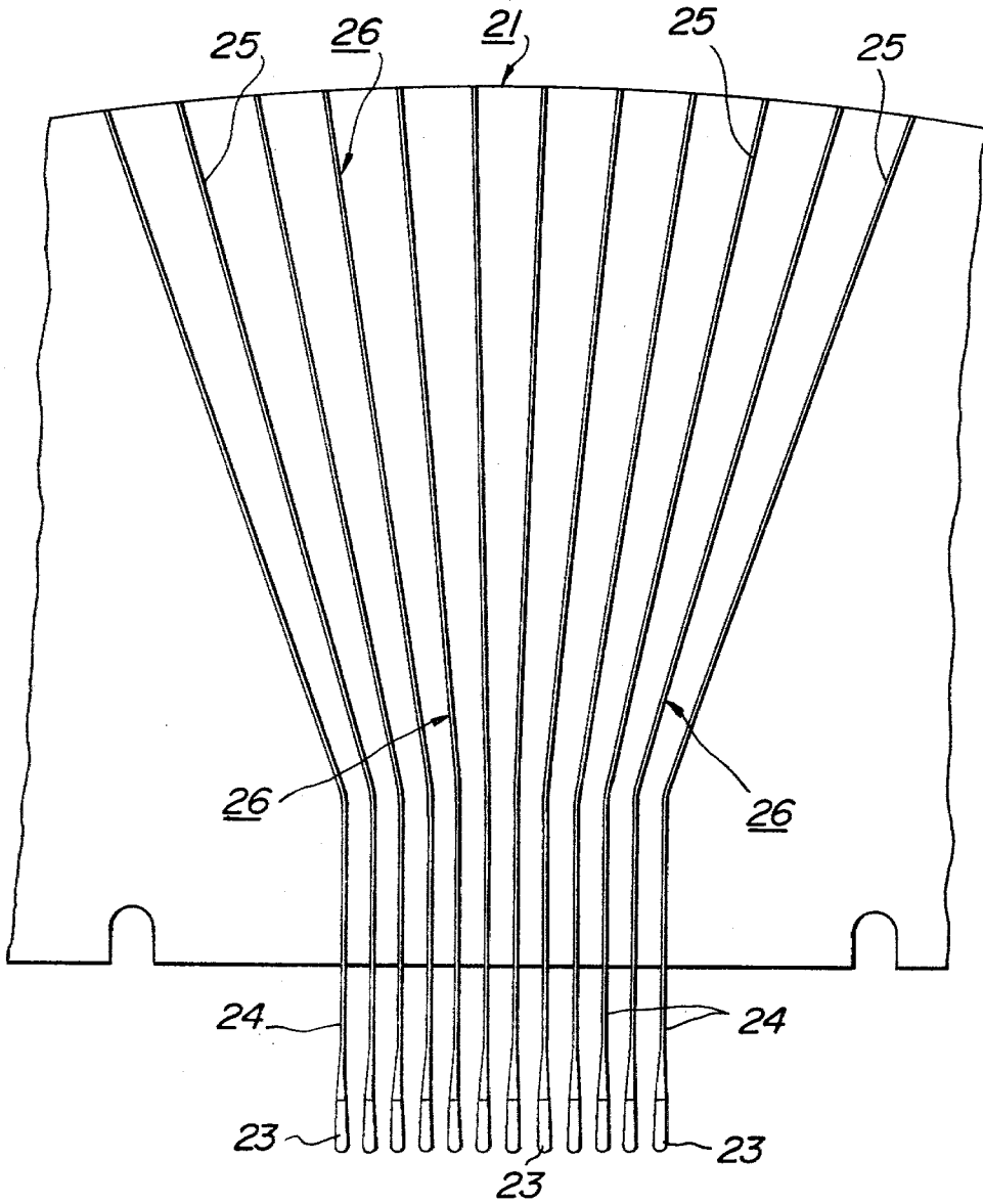
FIG. 8 PRIOR ART
