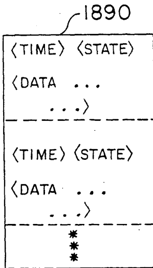
FIG. 85 SCHEDULE QUEUE
