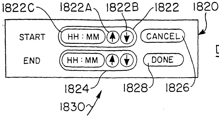
FIG. 85 SCHEDULE QUEUE
