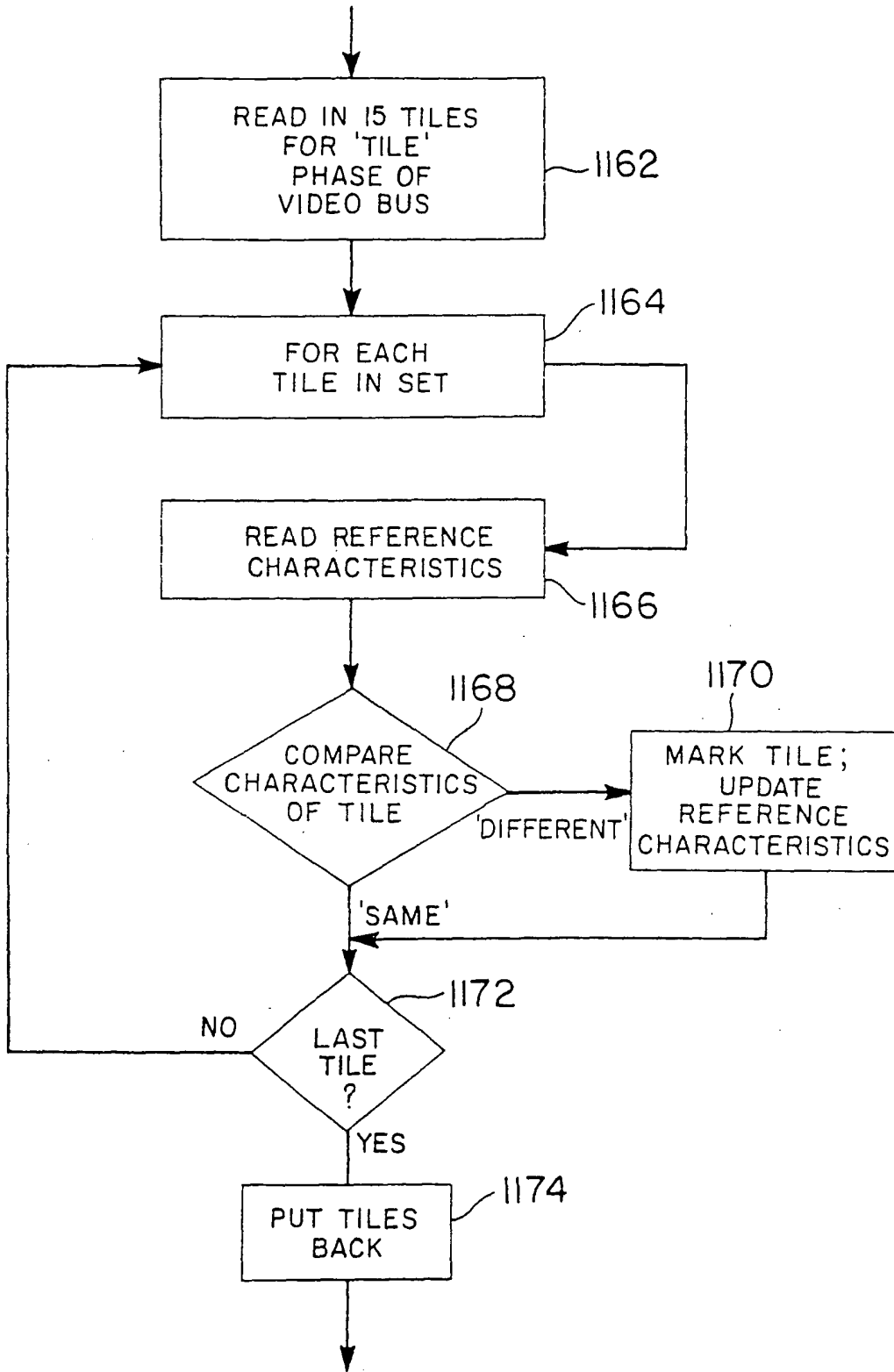
FIG. 42 TILE COMPARING
