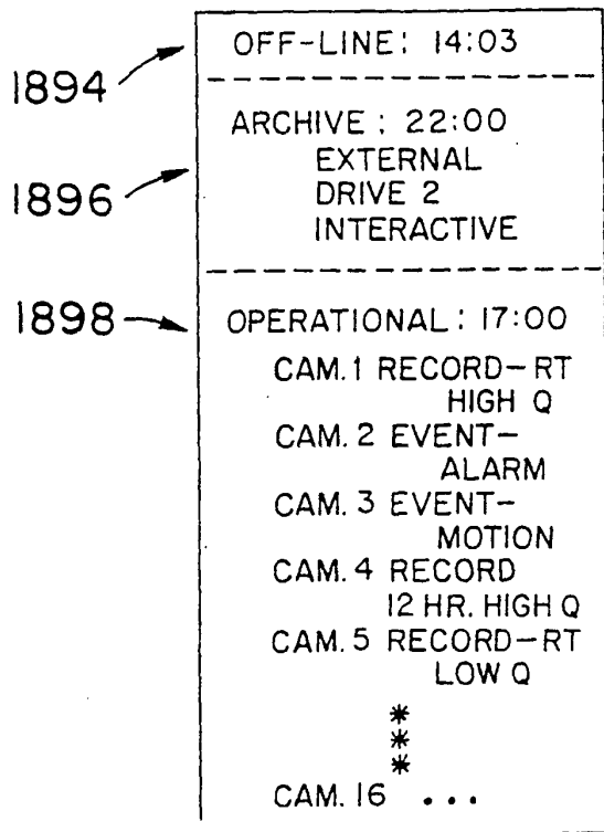
FIG. 86 SCHEDULE SCRIPT/TABLE
