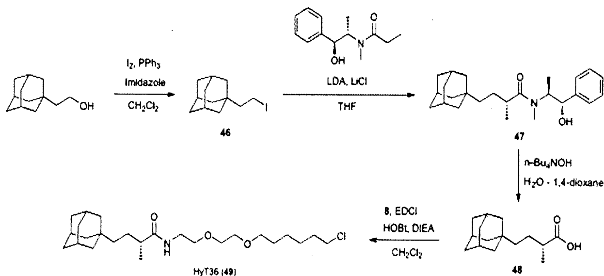
Scheme 12. Synthesis of HyT36 (49)
