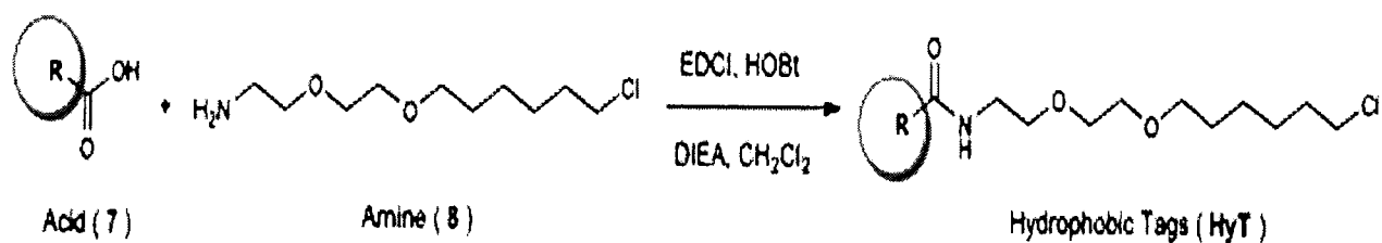
Scheme 1. General Synthetic Scheme for Hydrophobic Tags (Halotag)
