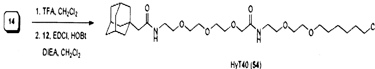
Scheme 14. Synthesis of HyT40 ( 54 )
