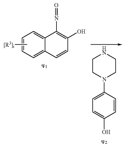
Reaction Sequence J
