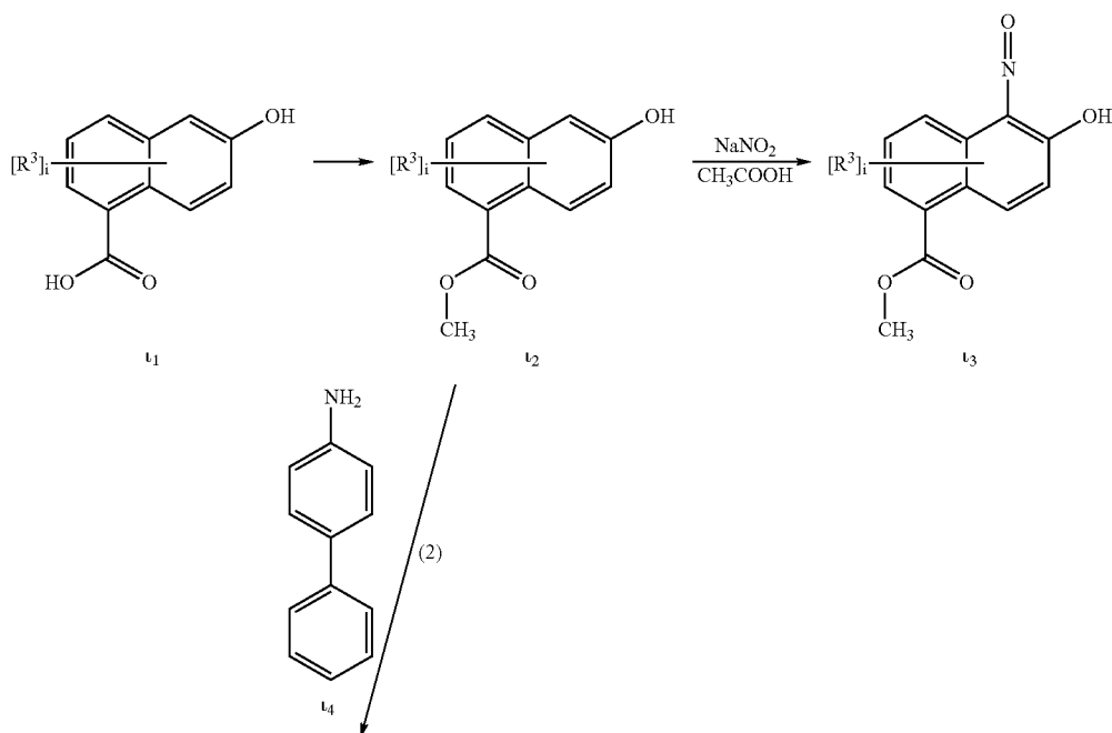
Reaction Sequence I
