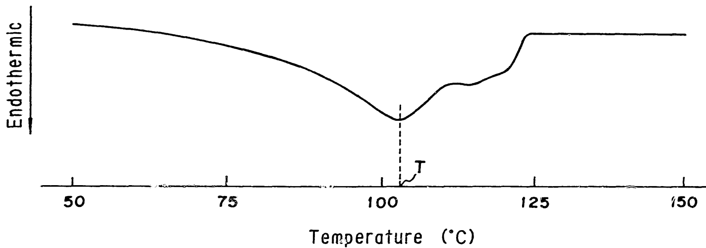
Endothermic Curve Measured by DSC (EX.2)
